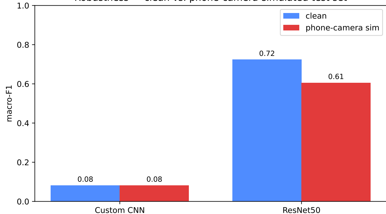
Robustness — clean vs. phone-camera-simulated test set
