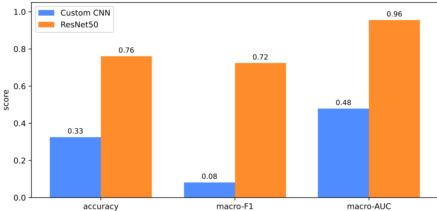
Model comparison — Custom CNN vs. ResNet50 (test set)
