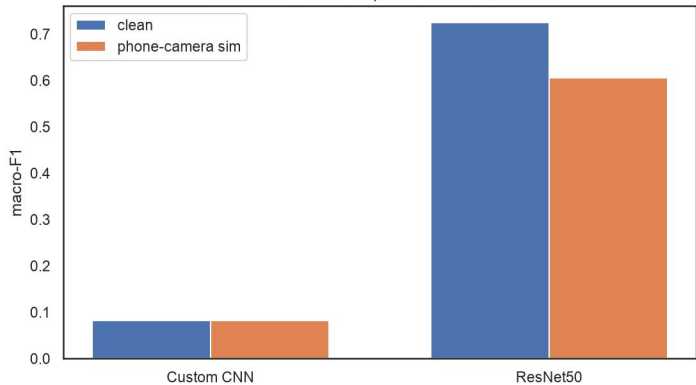
Robustness - clean vs. phone-camera simulation
