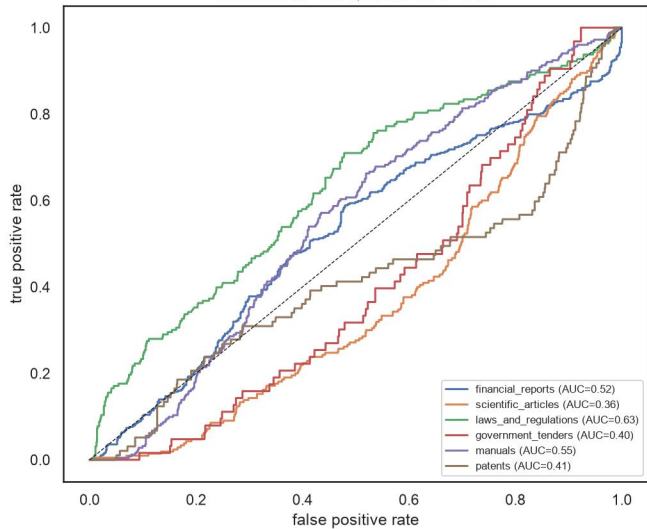
Custom CNN - ROC, macro-AUC=0.479
