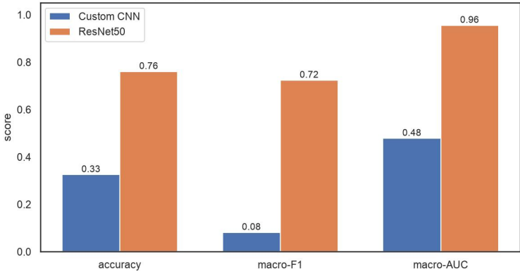
Model comparison - actual test-set scores
