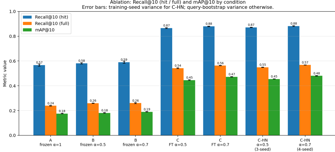
Figure 2: Ablation summary across the conditions. Bars show R@10 (hit-rate and full-Recall) and mAP@10. The dominant lift comes from fine-tuning (A/B \rightarrow C); hard-negative mining and \alpha = 0.7 over \alpha = 0.5 each add a smaller increment on top.
