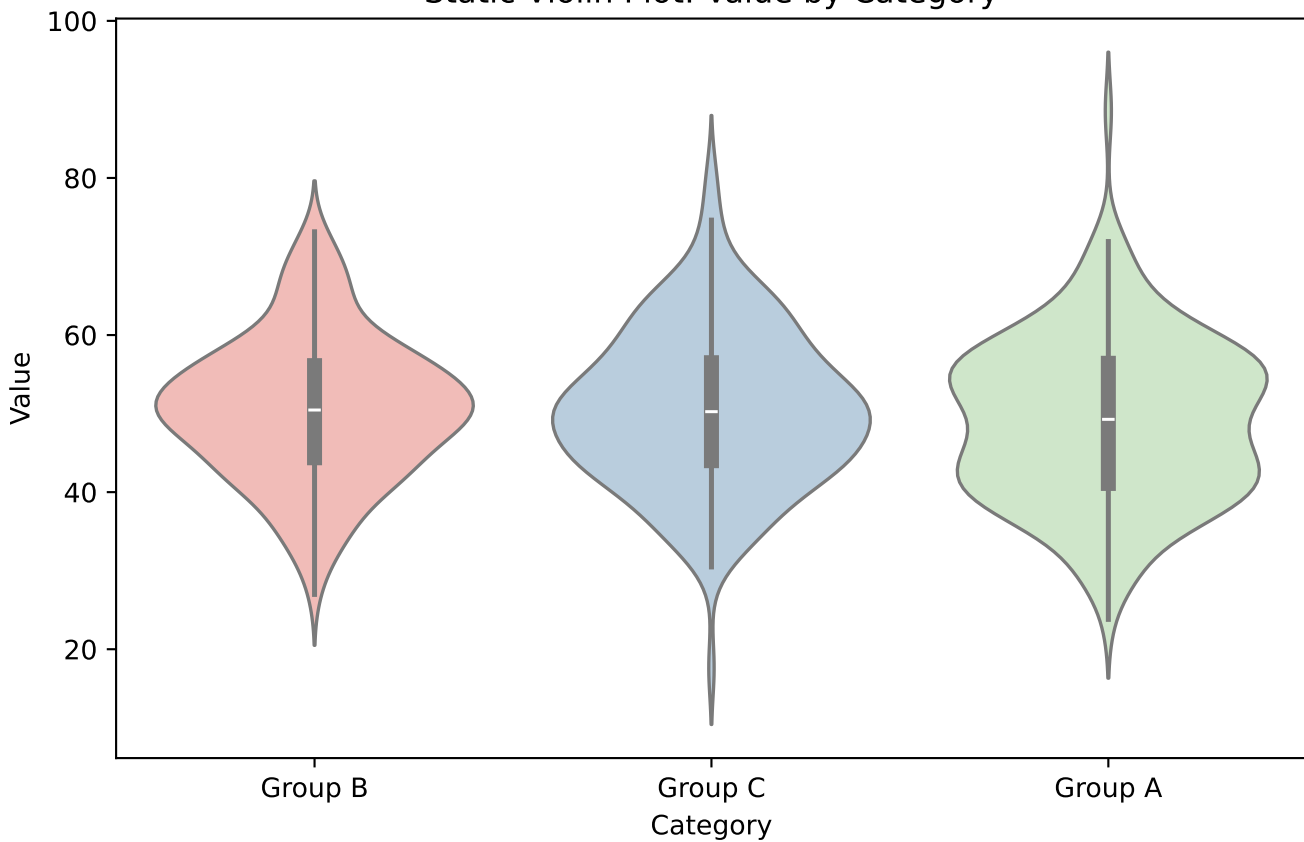
Static Violin Plot: Value by Category
