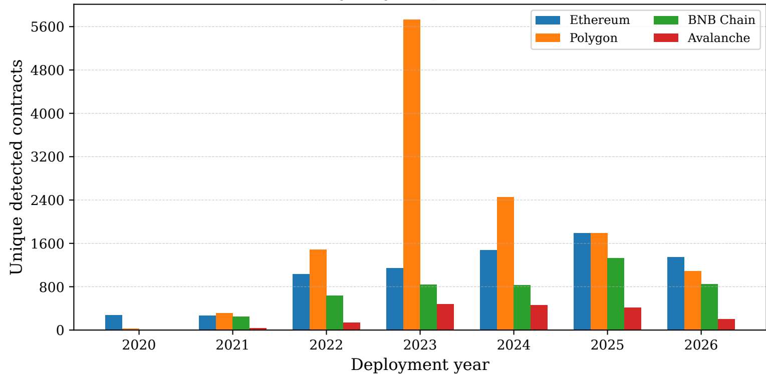
ERC-1271: yearly adoption across chains
