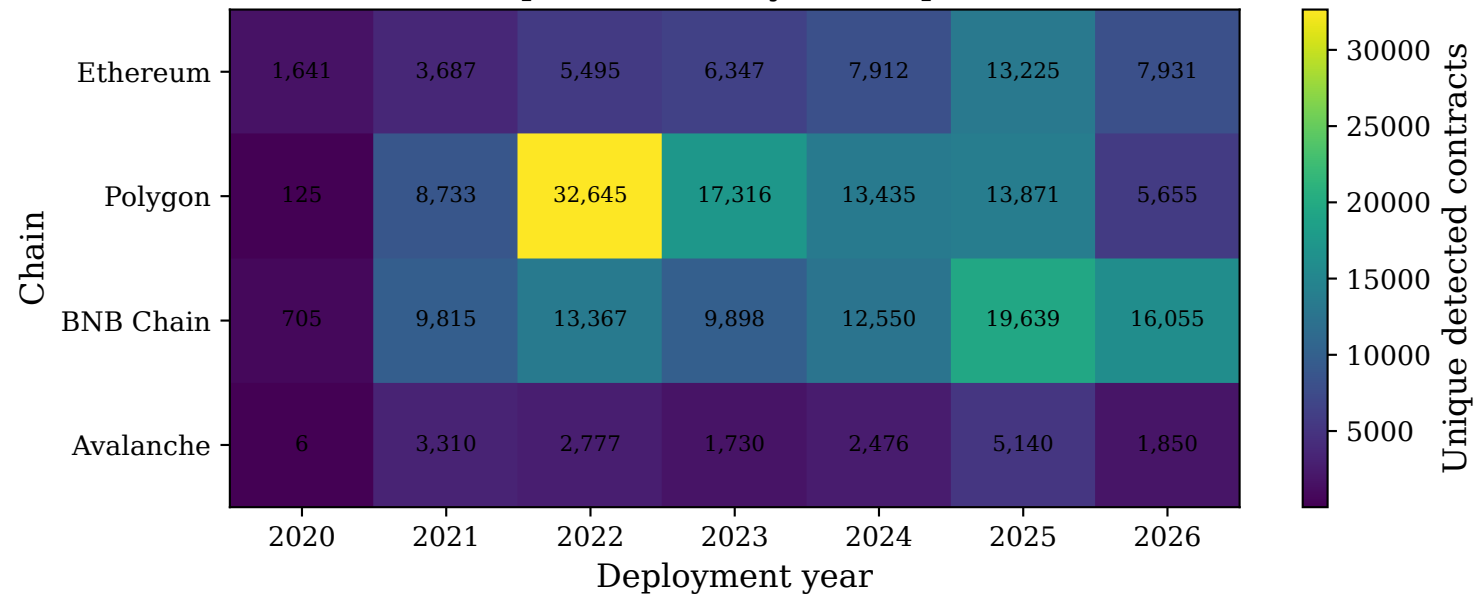
ERC-2612 permit: chain-year adoption matrix
