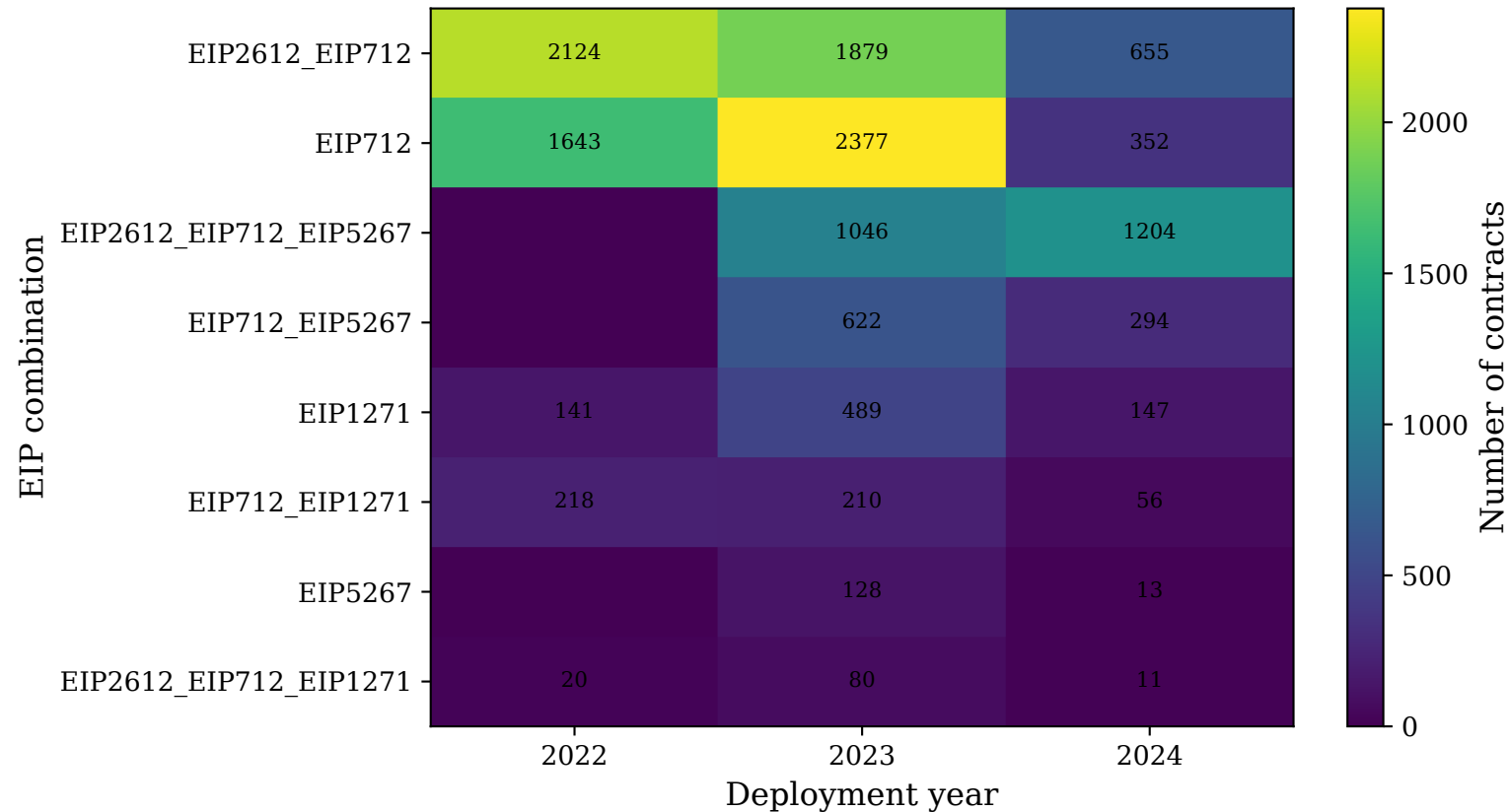
Dominant EIP combinations over time
