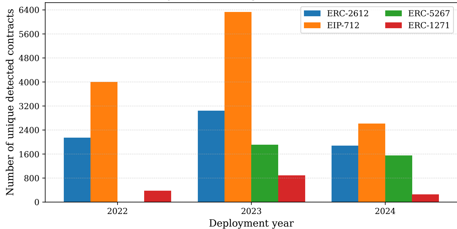
Yearly adoption of signature-related EIPs
