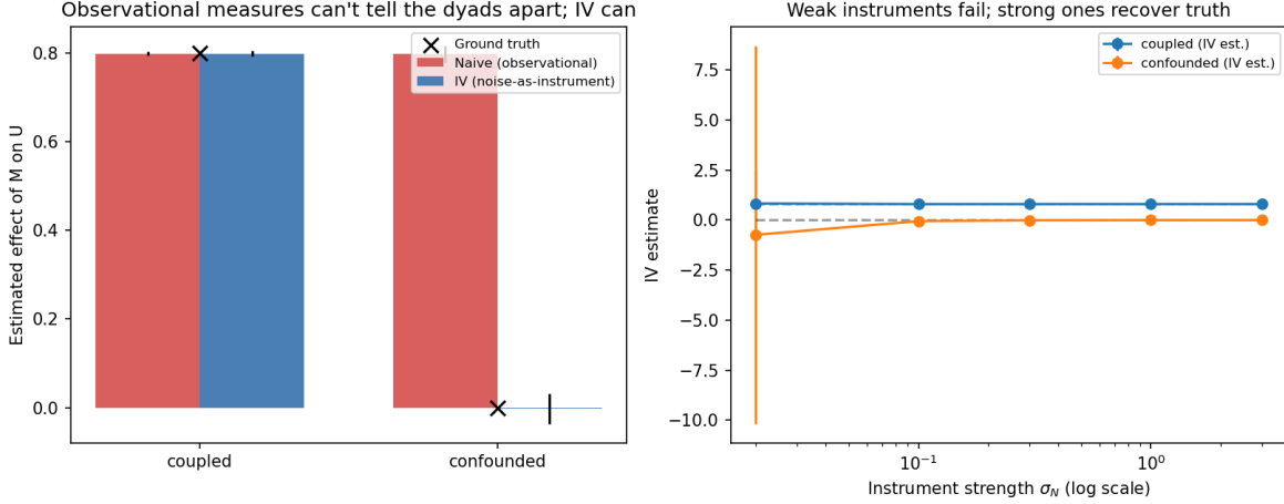
Figure 2: Left: the naive observational regression cannot separate the coupled dyad from the confounded one — both return the same estimate, and only the coupled dyad’s matches ground truth by coincidence. The instrumental estimate recovers each dyad’s true value, including the confounded dyad’s true zero. Right: the instrument degrades gracefully as its strength \sigma_N falls, motivating the first-stage diagnostic rather than an assumed-valid instrument.
