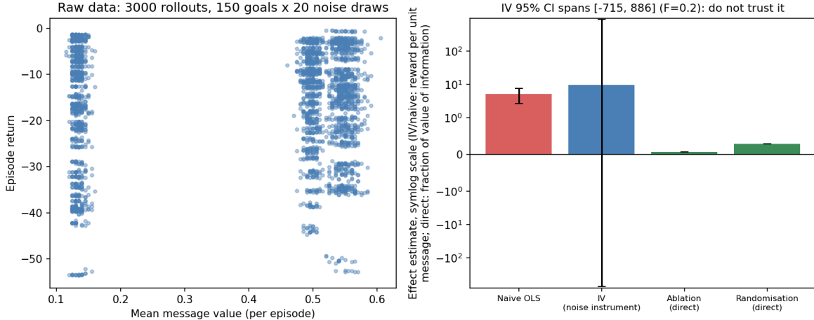
Figure 3: Left: raw rollouts on the real trained system, message value clustering by goal rather than varying smoothly with noise — visible evidence of the low within-goal variance the text describes. Right: naive OLS and the IV estimate are both far from the ablation/randomisation-based direct estimates of the value of information, and the IV estimate’s error bar is enormous — the first-stage diagnostic ( F = 0.2 ) correctly flags this estimate as unusable rather than letting a point estimate mislead.
