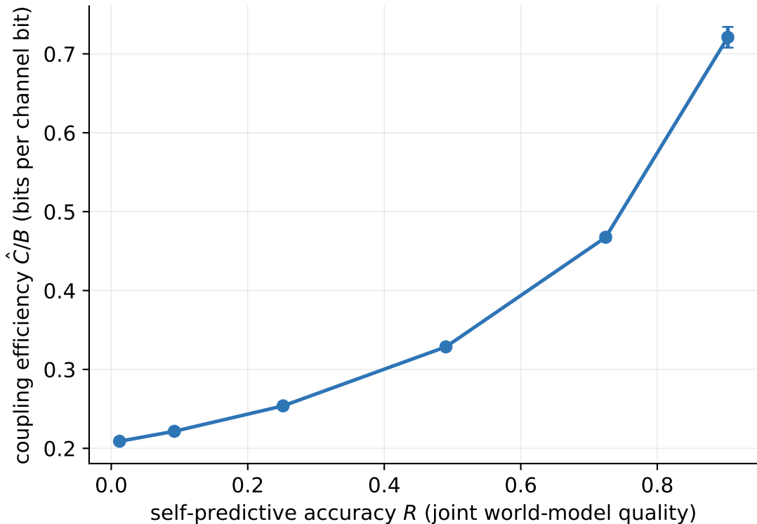
Prediction 2 -- better world models couple more per bit (Pearson r = 0.94 )
