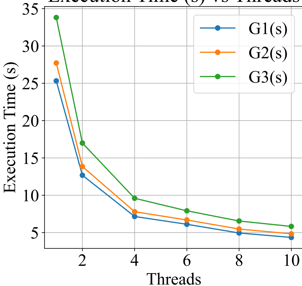
Execution Time (s) vs Threads
