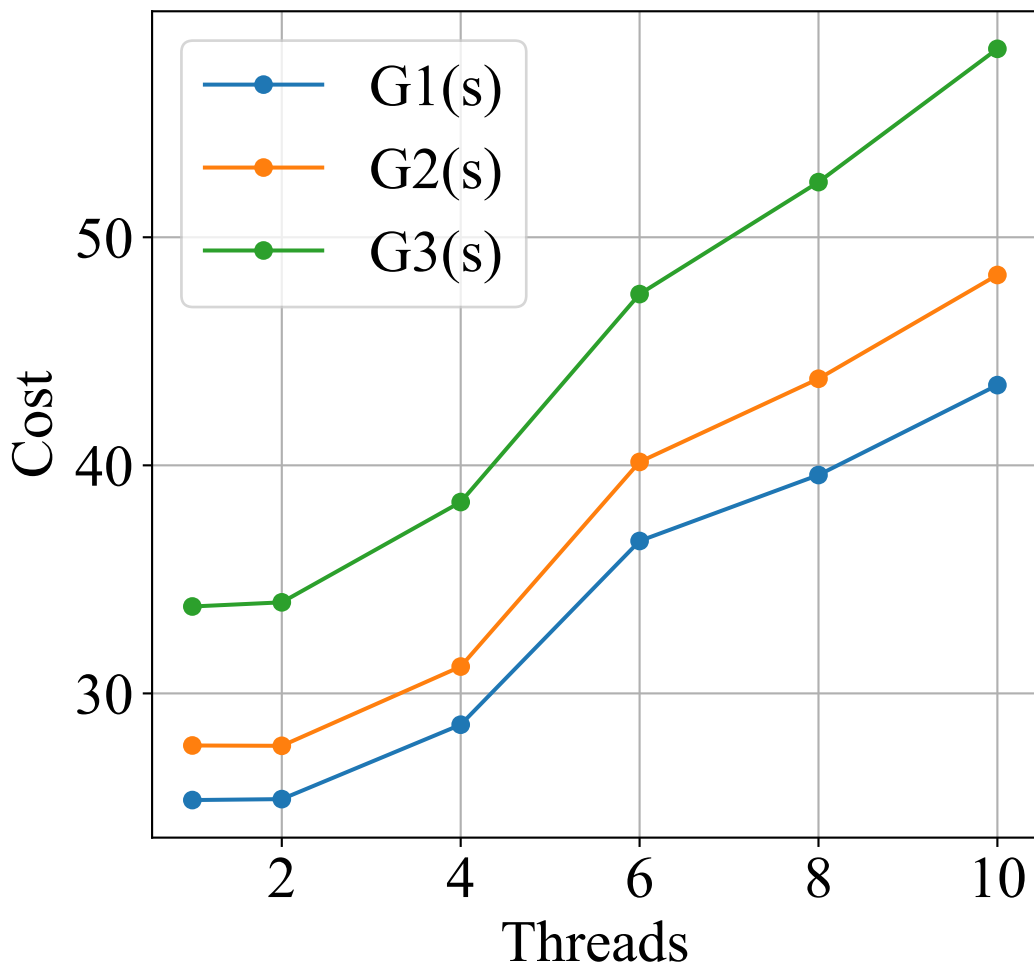
Cost vs Threads
