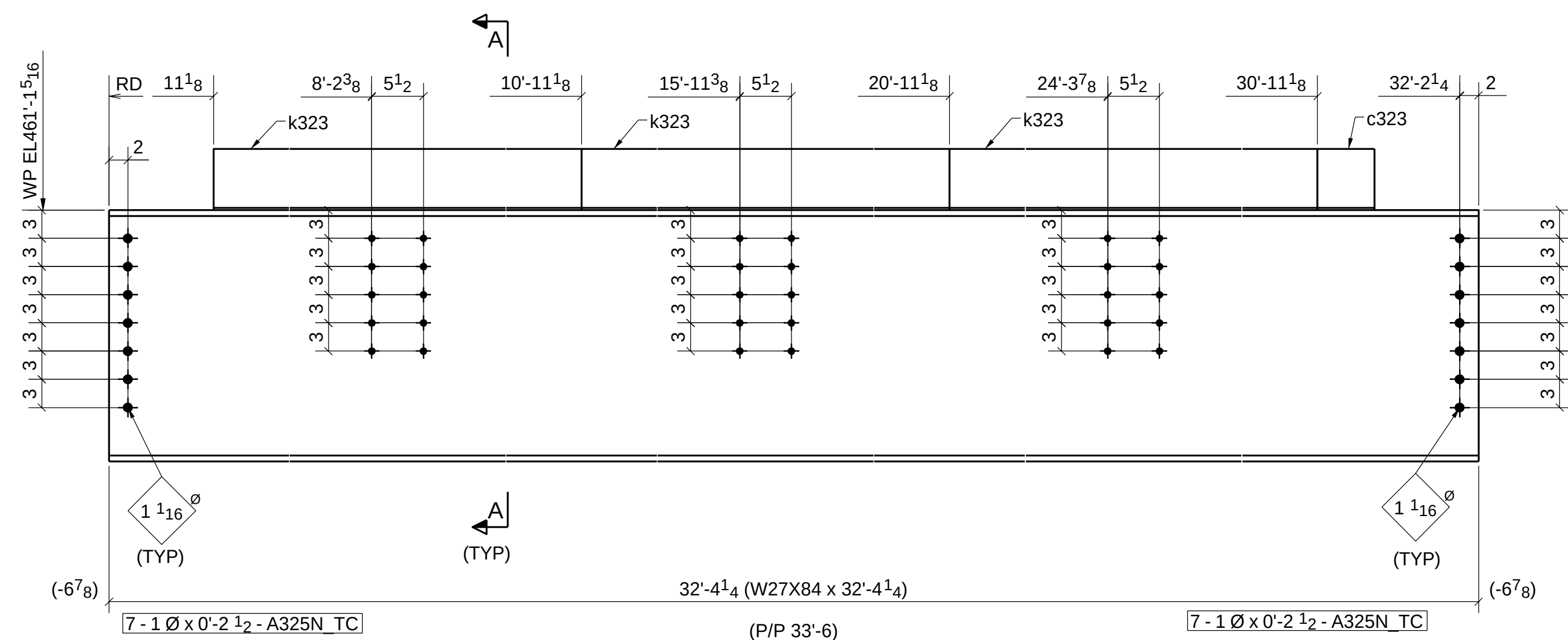
ONE ~ BEAM ~ 323B1 (ONE @ E302) (NO PAINT)
