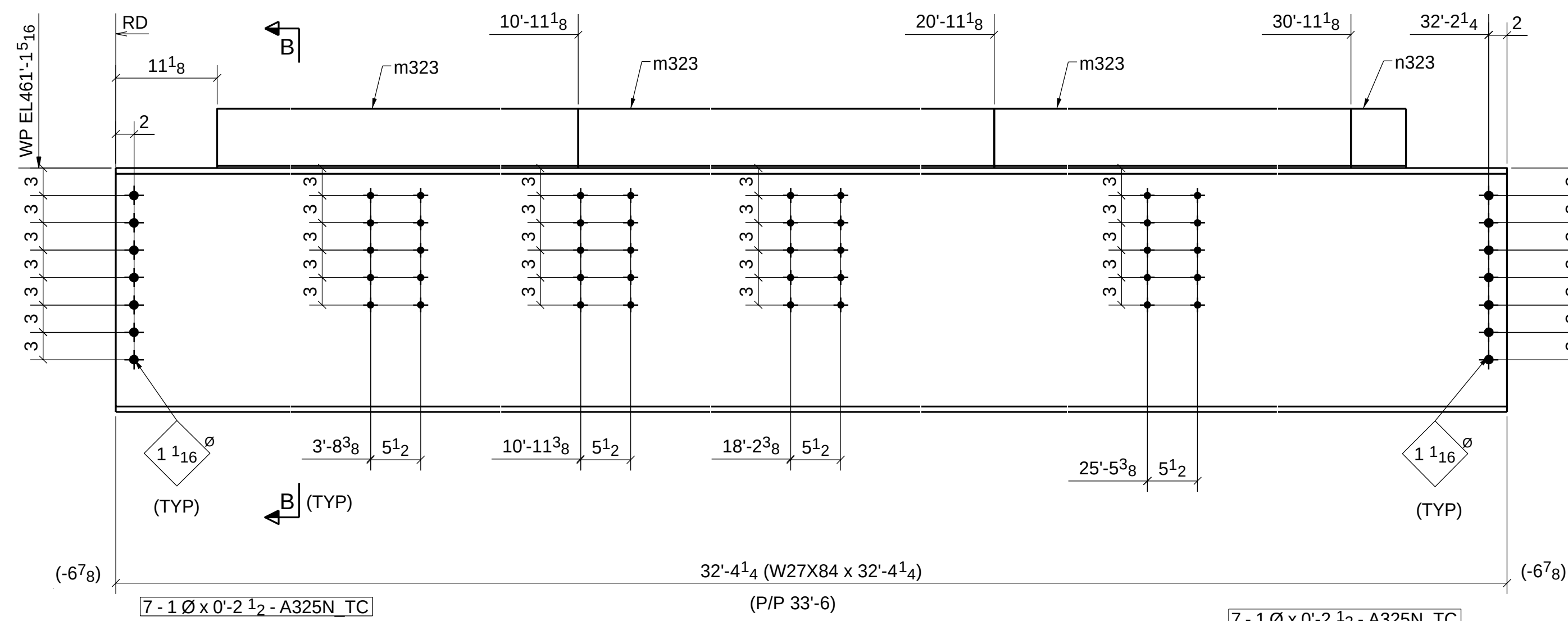
ONE ~ BEAM ~ 323B3 (ONE @ E302) (NO PAINT)
