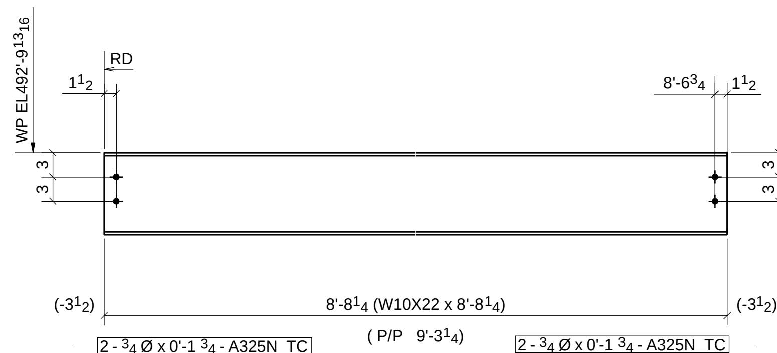
ONE ~ BEAM ~ 323B2 (ONE @ E307) (NO PAINT)
