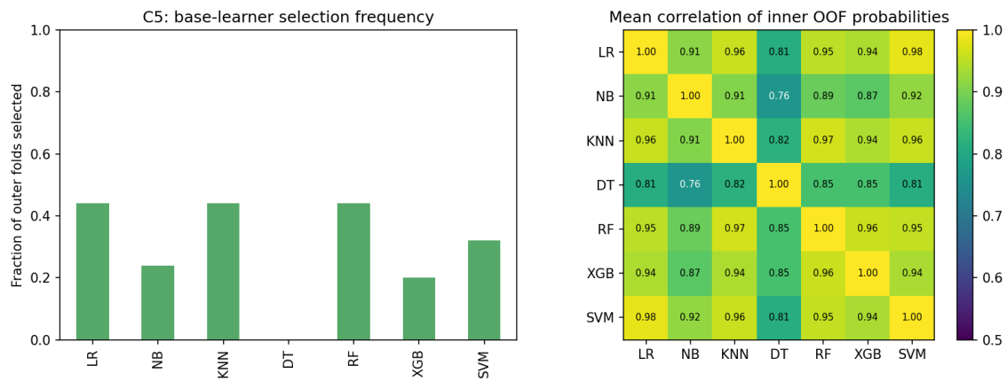
Fig. 8. Left: fraction of outer folds in which each tuned learner is selected by C5. Right: mean correlation between inner out-of-fold probabilities.
