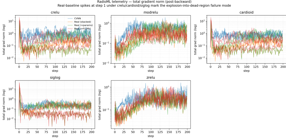
Figure 4: RadioML telemetry — total gradient norm post-backward, log y -axis, one panel per activation. Real-baseline spikes at step 1 under crelu / cardioid / siglog mark the explosion-into-dead-region failure mode that produces the inflated gaps in Section 3; under modrelu and zrelu no such spikes occur and the gap collapses to \pm 3 pp.
