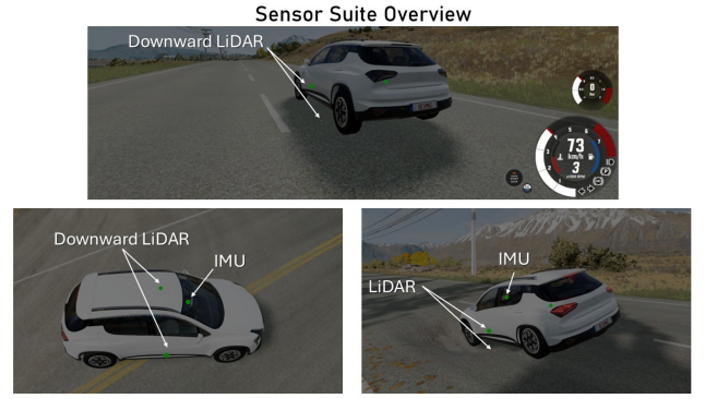
Fig. 1. Virtual sensor placement within BeamNG.tech. Dual downward-facing LiDAR sensors at left/right wheel tracks ( \pm 0.85 m lateral offset) record road elevation h(x) ; a dashboard-mounted AdvancedIMU records 3-axis acceleration and angular velocity.
