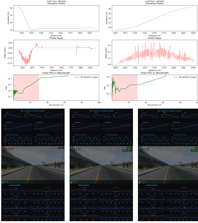
Fig. 2. Polygon-mesh tessellation artifact and Curvature-Adaptive Correction. (a) Power Spectral Density (PSD) analysis: flat road (left column) shows negligible PSD energy in the IRI-sensitive band (1–30 m); sloped road (right column) shows severe high-frequency slope oscillations concentrated in the 1–10 m band due to dihedral facet edges. (b) Uncorrected elevation profile on a sloped highway ramp, inflating computed IRI to \sim 15 m/km. (c) Corrected profile after curvature-adaptive blending ( \alpha > 0 when \kappa > \kappa_{\text{thresh}} ); IRI returns to physically valid baseline while preserving genuine roughness on flat sections. (d) Sensor placement reference (dual LiDAR + dashboard IMU).
