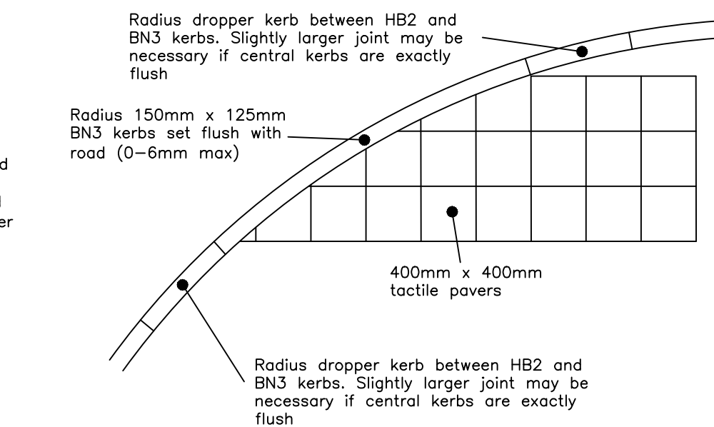
Typical Dropped Kerb Detail for Tactile Paving N.T.S.
