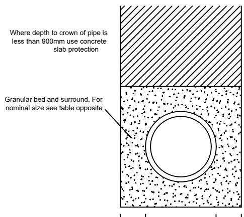
CLASS S PIPE BED AND SURROUND
