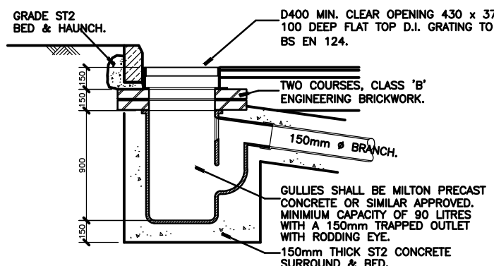
ROAD GULLY DETAIL.
