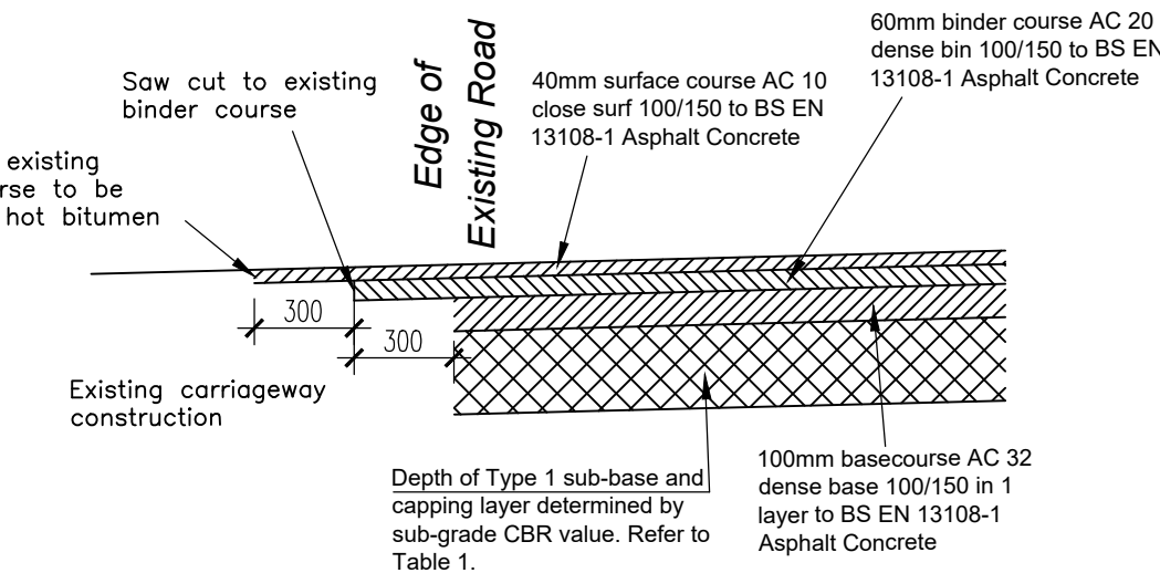
New Estate Road Tie-in to Existing Road
