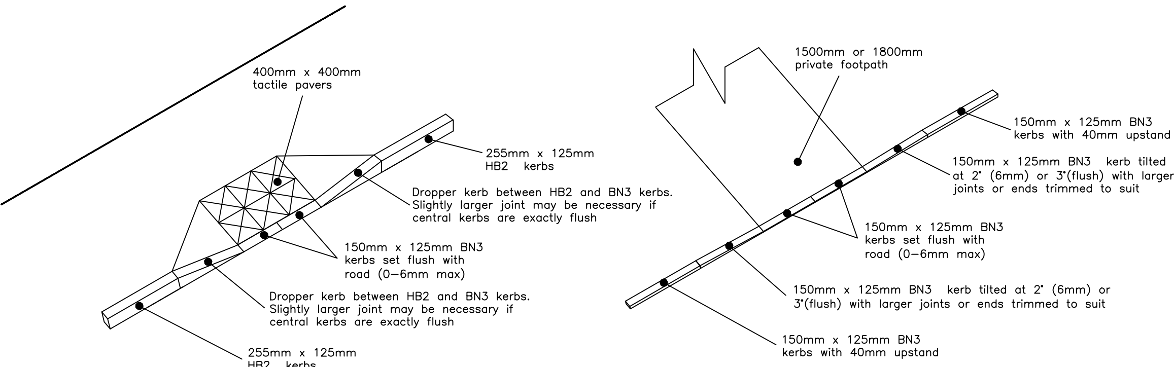
Typical Dropped Kerb Detail for Tactile Paving N.T.S.
