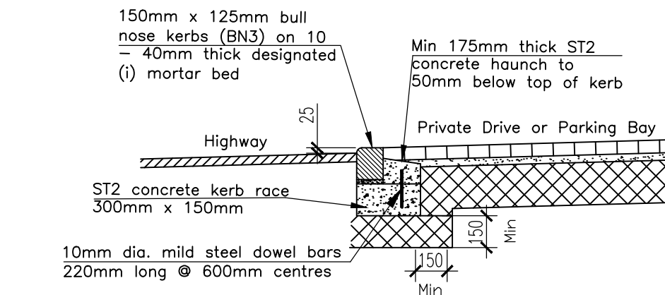
Upstand on Bull Nose Kerbs to be 25mm between Adoptable Road and Private Drive or Parking Bay
