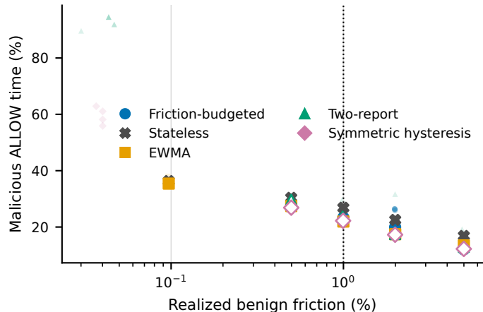
(a) Security-friction
