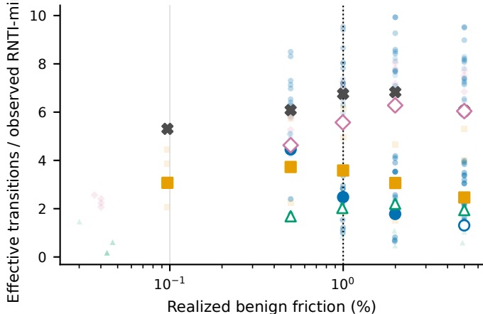
(b) Stability-friction
