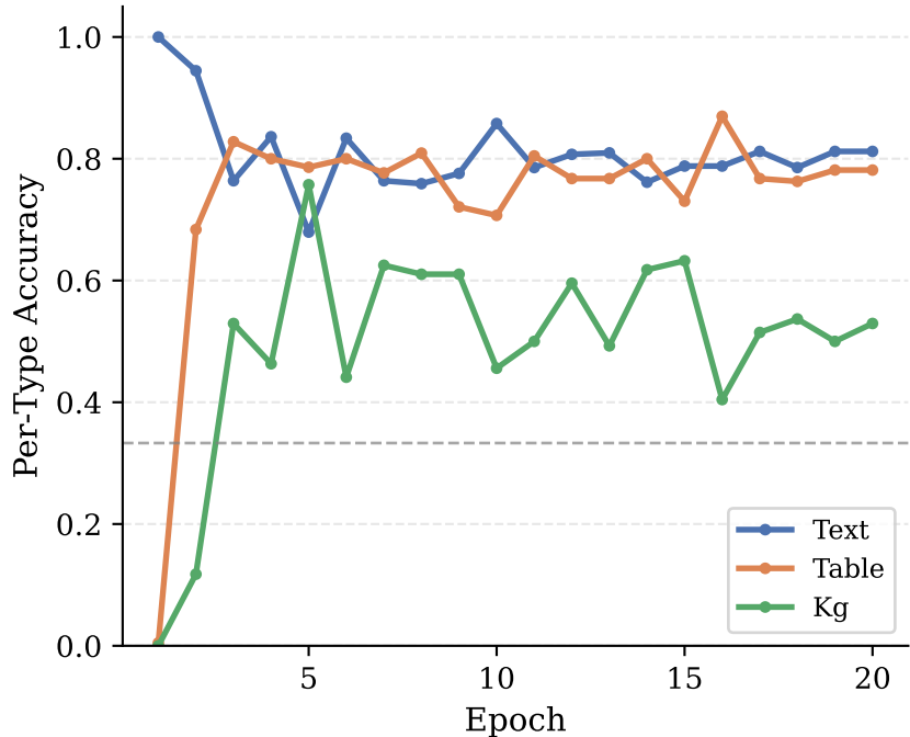
(b) K=3 Per-Type (seed 42)
