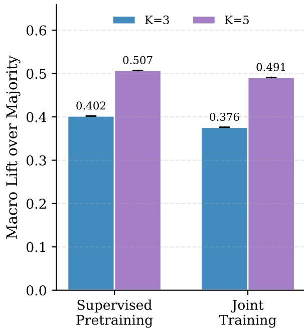
(b) Lift over Majority Baseline (dev)
