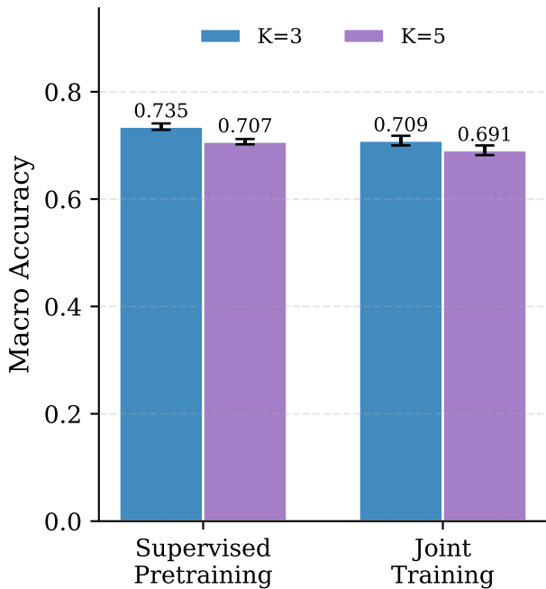
(a) Routing Macro Accuracy (dev)
