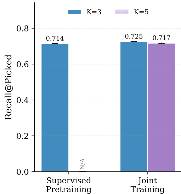
(c) Recall@Picked (test)
