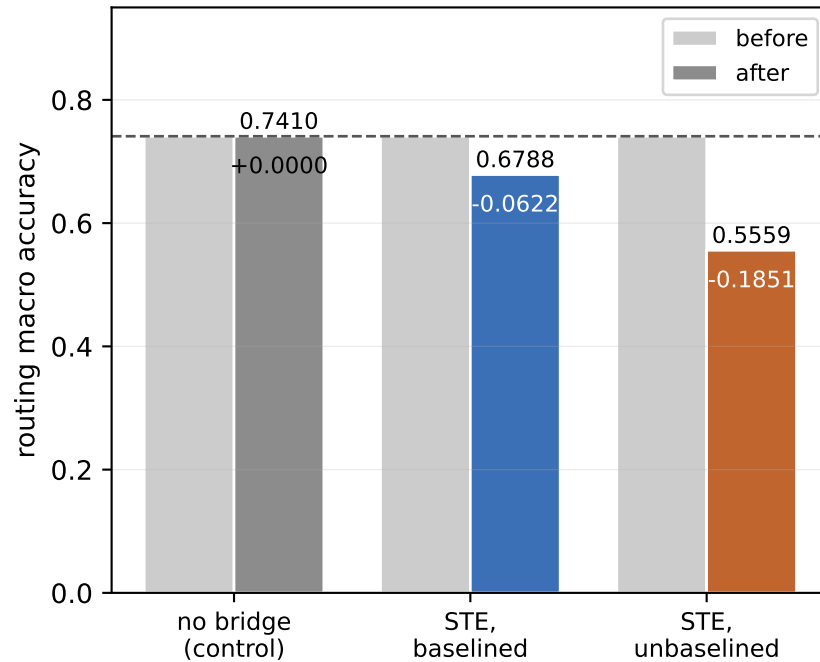
(b) Effect on routing (supervised checkpoint start)
