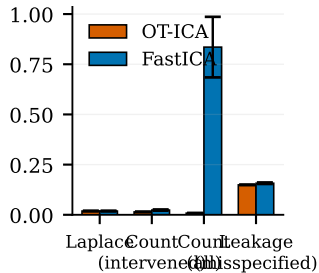
Amari error (lower better)
