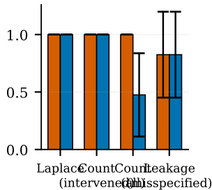
target accuracy (higher better)
