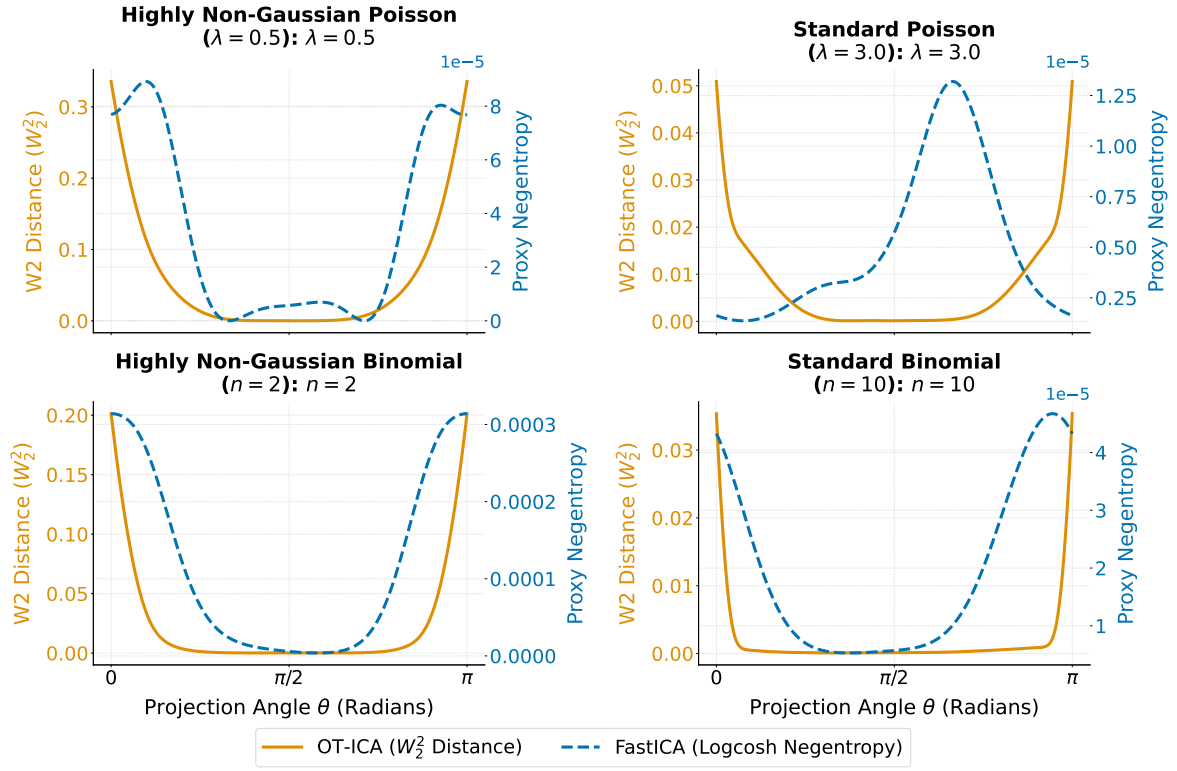
Figure 8: W_2^2 and logcosh optimization landscapes for two-source Poisson and Binomial mixtures across parameterizations. The W_2^2 landscape retains a non-zero signal throughout (confirming the contrast is present), but the step-function geometry of discrete CDFs creates flat plateaus where the gradient evaluates to near-zero, stalling gradient-based solvers. The logcosh landscape degenerates to near-zero for standard count-based parameterizations, indicating a fundamental contrast failure.
