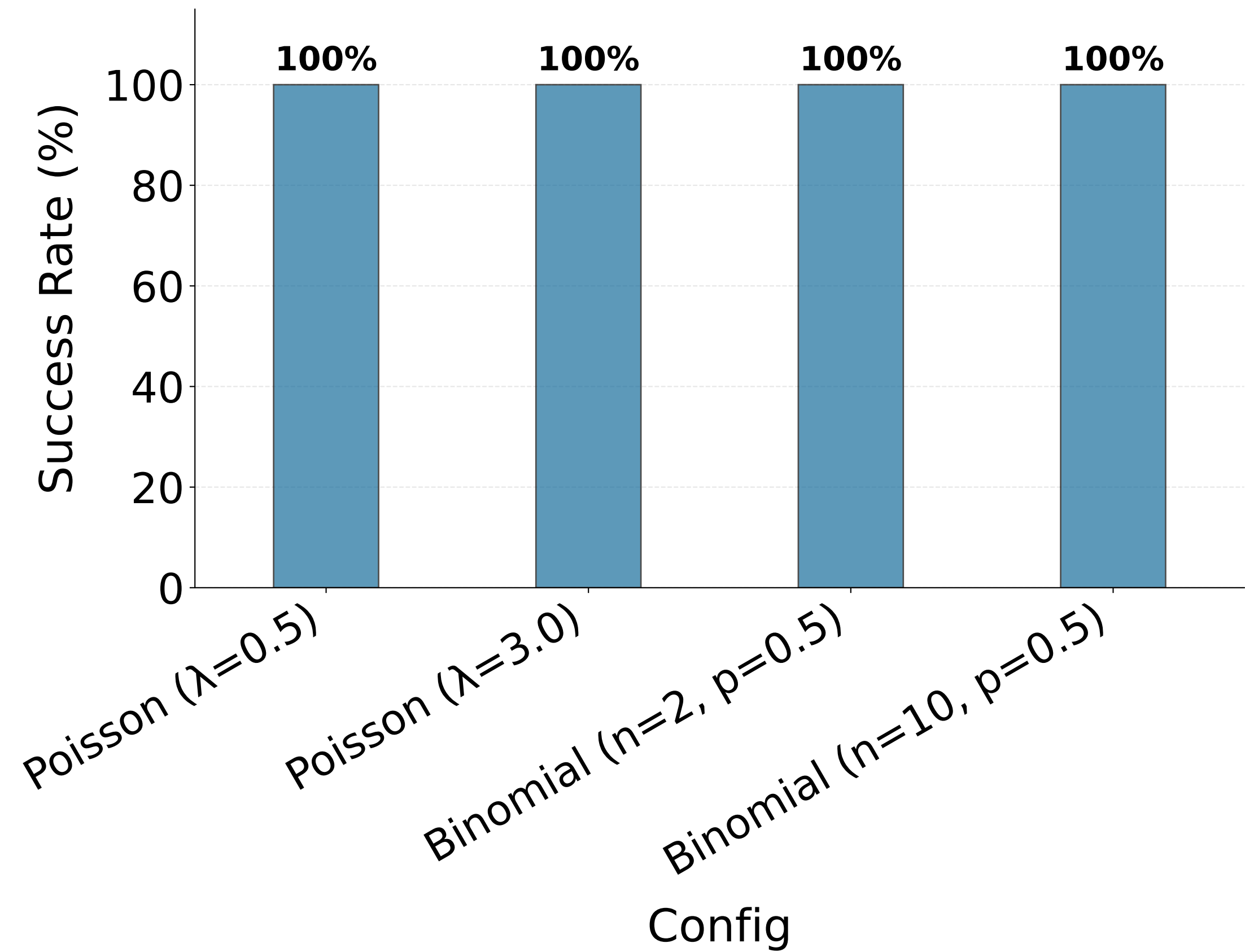
FastICA Convergence: Discrete
