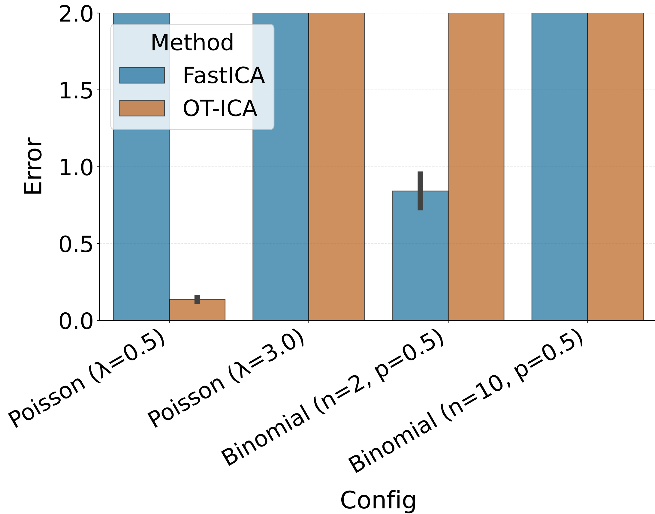
Amari Error: Discrete
