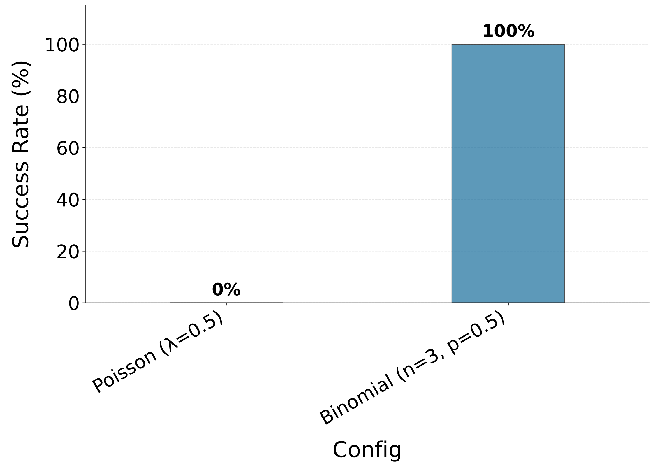
Convergence Rate: Harsh Discrete (FastICA Only)
