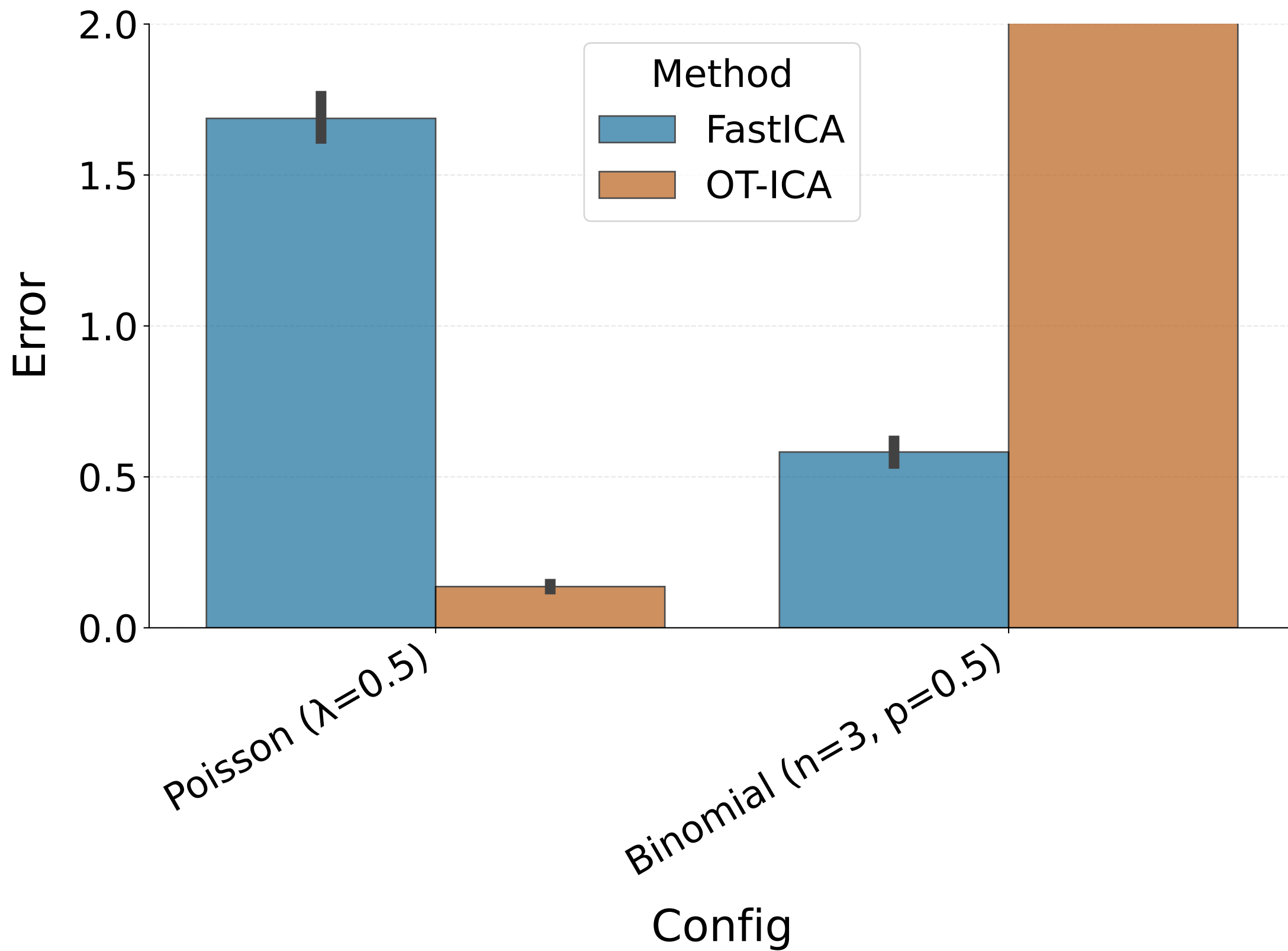
Amari Error: Harsh Discrete (Lower is Better)
