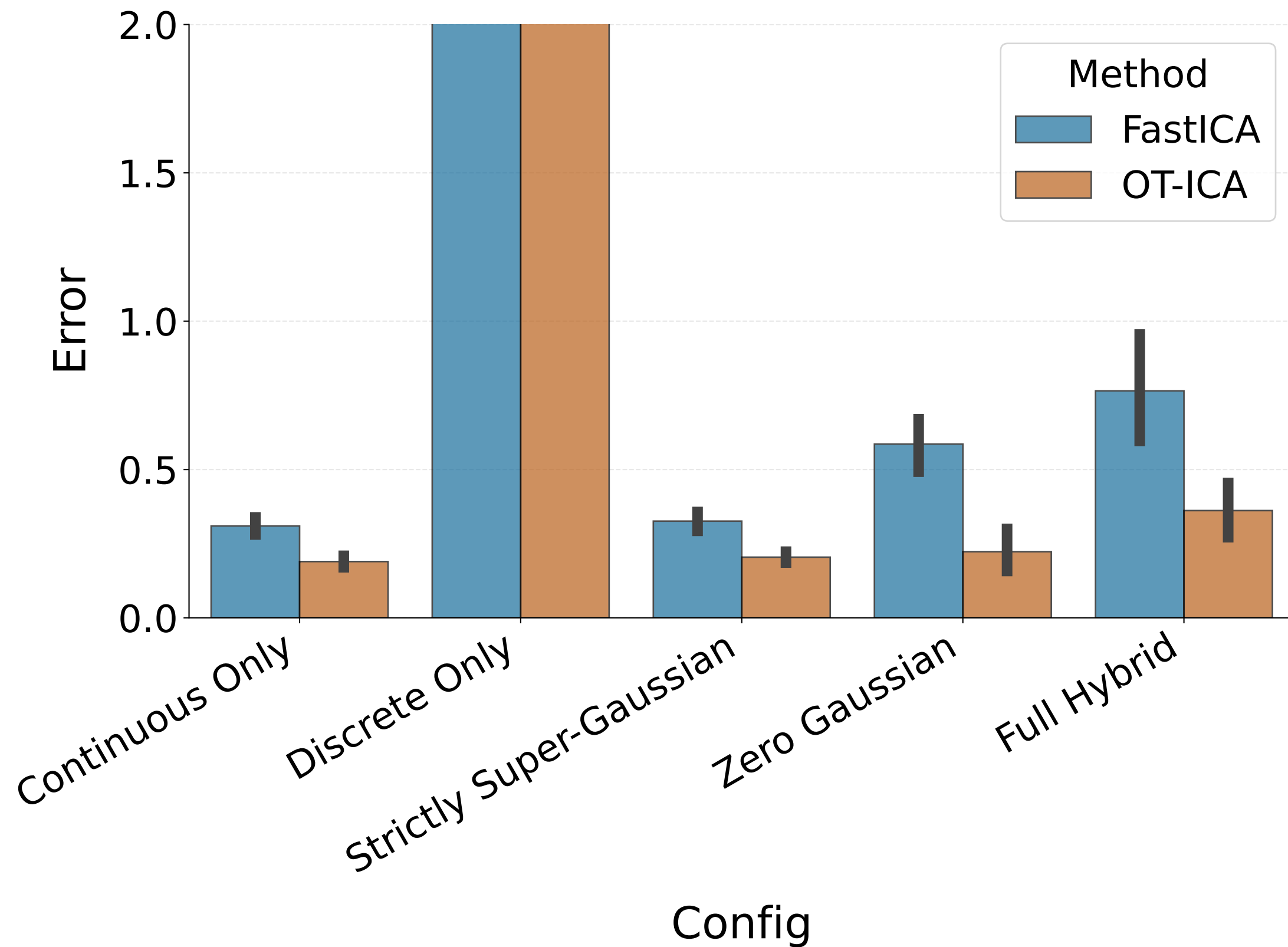
Amari Error: Sub-Pool Ablation (Lower is Better)
