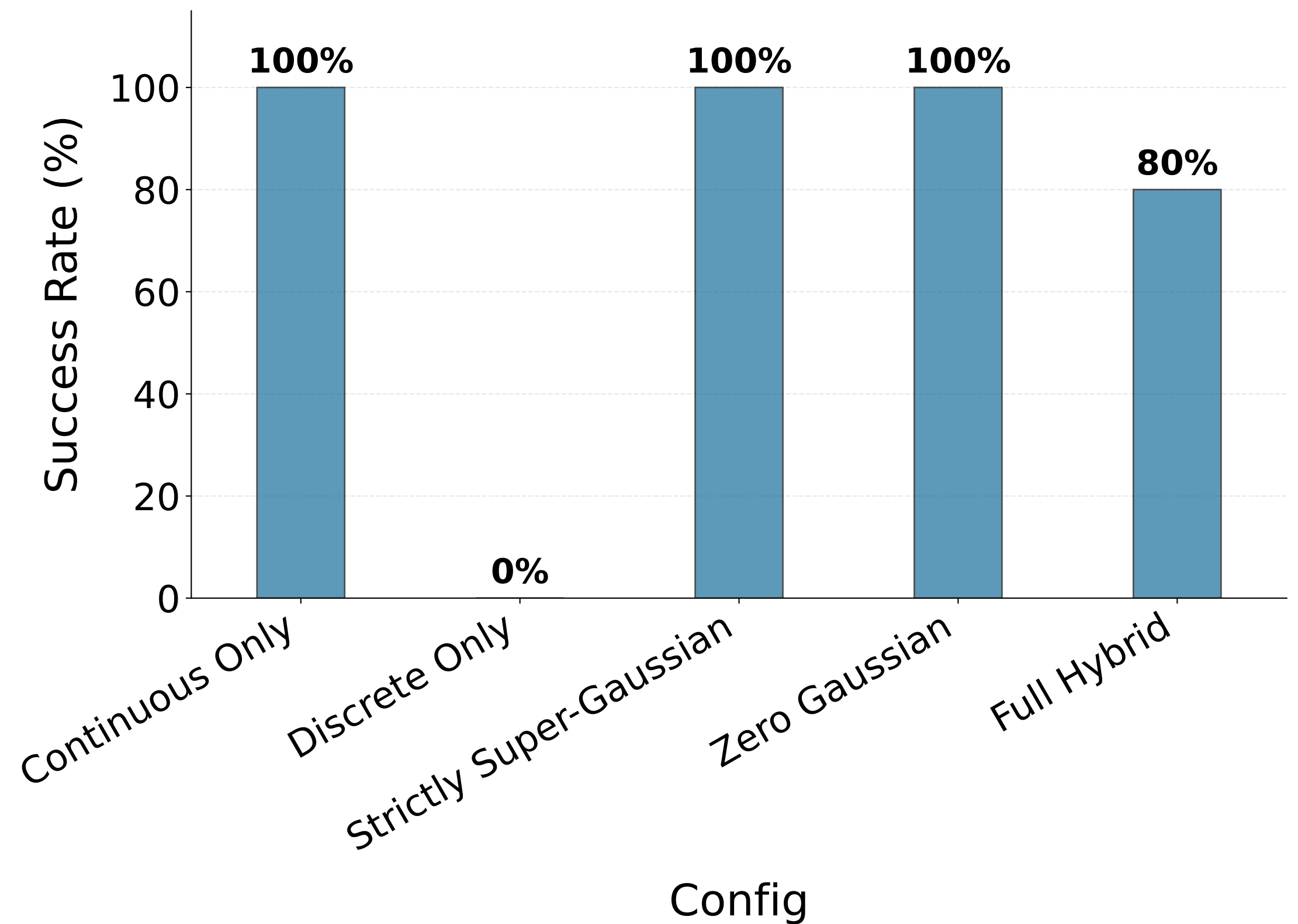
Convergence Rate: Sub-Pool Ablation (FastICA Only)
