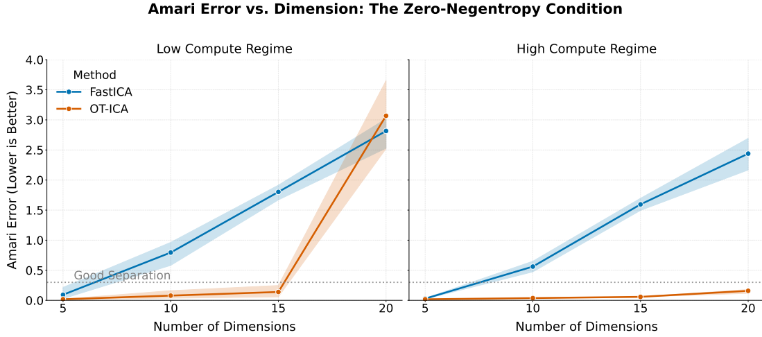
Figure 9: Amari error comparison for an engineered zero-negentropy distribution across Low and High compute regimes. FastICA’s error scales with dimension as the proxy gradient vanishes, crossing the good separation threshold ( E = 0.3 ). OT-ICA maintains good separation till higher dimensions depending on compute regime.
