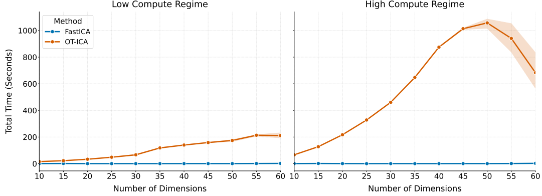
Figure 12: Total execution time (in seconds) for FastICA and OT-ICA across dimensions.
