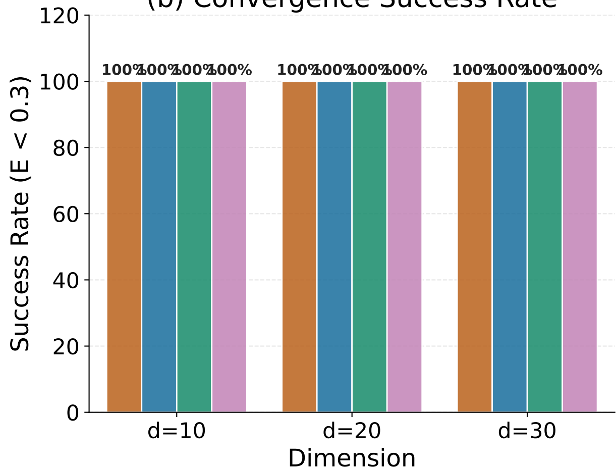
(b) Convergence Success Rate
