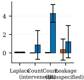
\|\hat{H} - H\|_F (lower better)
