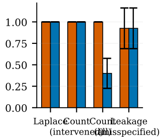
target accuracy (higher better)
