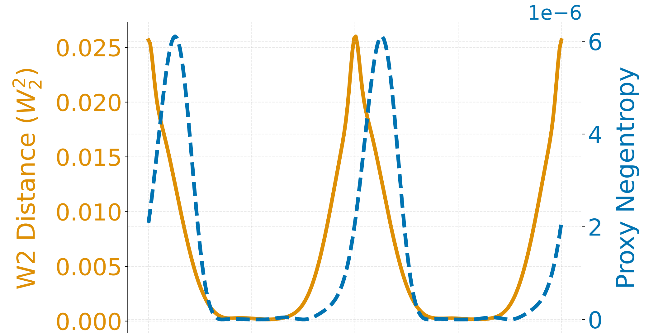
(II) Less Non-Gaussian Poisson ( \lambda = 3.0 ): \lambda = 3.0
