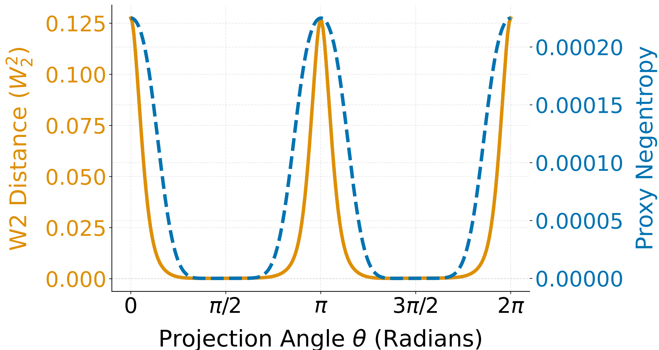
(III) More Non-Gaussian Binomial ( n = 2 ): n = 2
