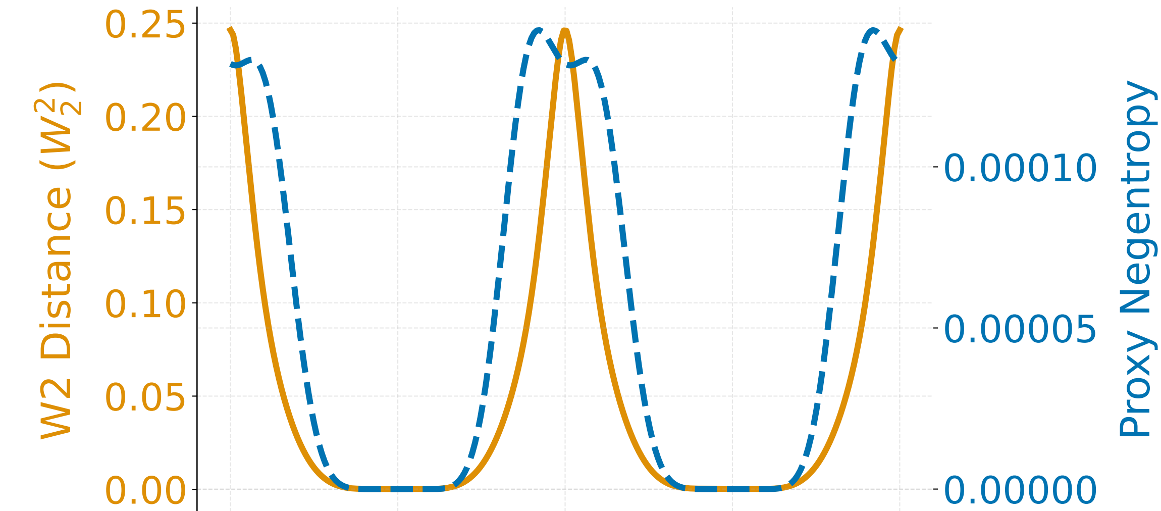
(I) More Non-Gaussian Poisson ( \lambda = 0.5 ): \lambda = 0.5
