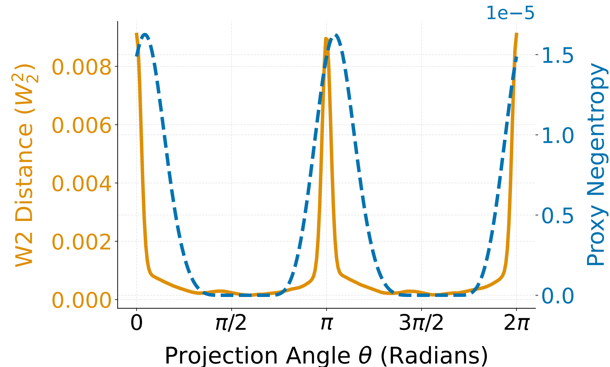
(IV) Less Non-Gaussian Binomial ( n = 10 ): n = 10
