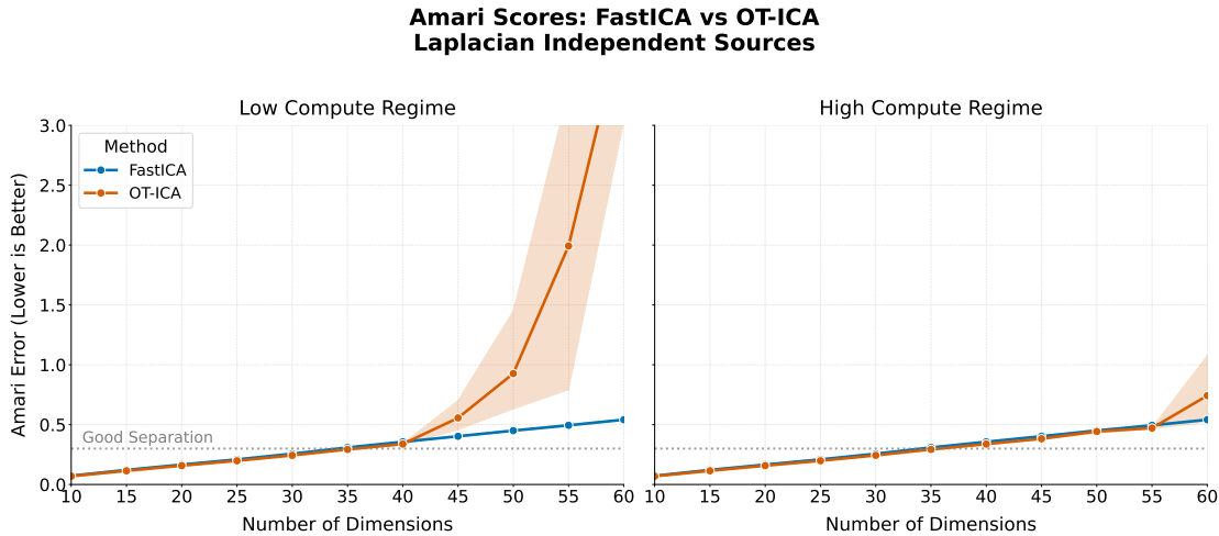
Figure 5.9: Amari error comparison across dimensions for Laplacian sources.
