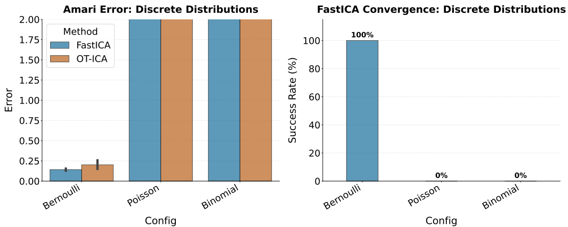
Figure 5.6: Amari error for discrete mixtures. Both algorithms separate binary data (Bernoulli) but exhibit higher error on multi-step count data (Poisson, Binomial).
