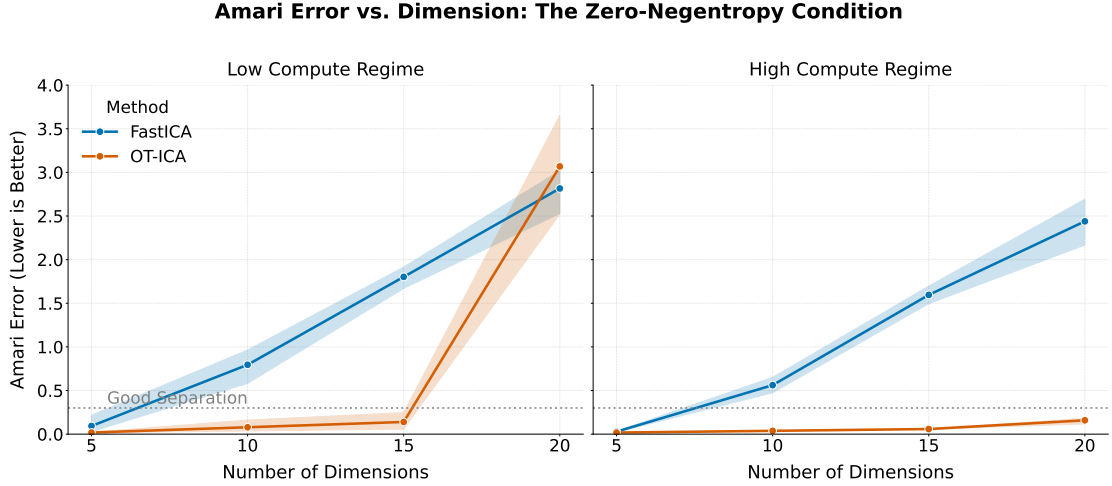
Figure 5.3: Amari error comparison for the zero-negentropy distribution up to d = 20 .
