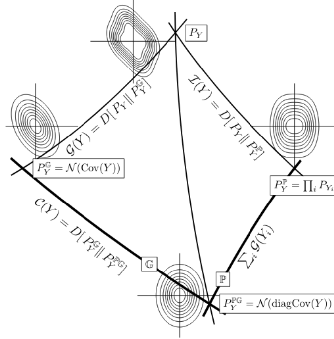
Figure 4: The Pythagorean geometry of Independent Component Analysis. Figure from ?.
