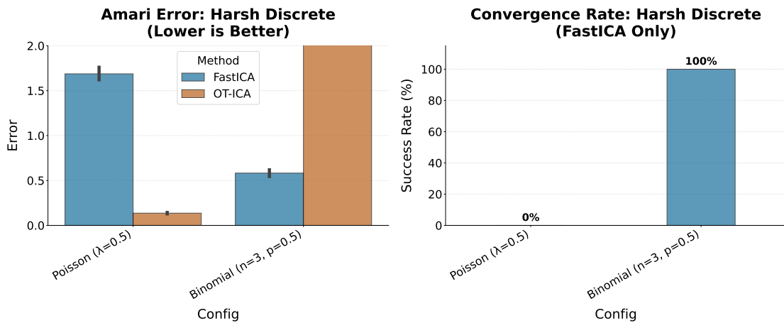
Figure 5.8: Amari Error for skewed discrete parameterizations. OT-ICA achieves separation on the Poisson distribution but does not converge on the symmetric Binomial.
