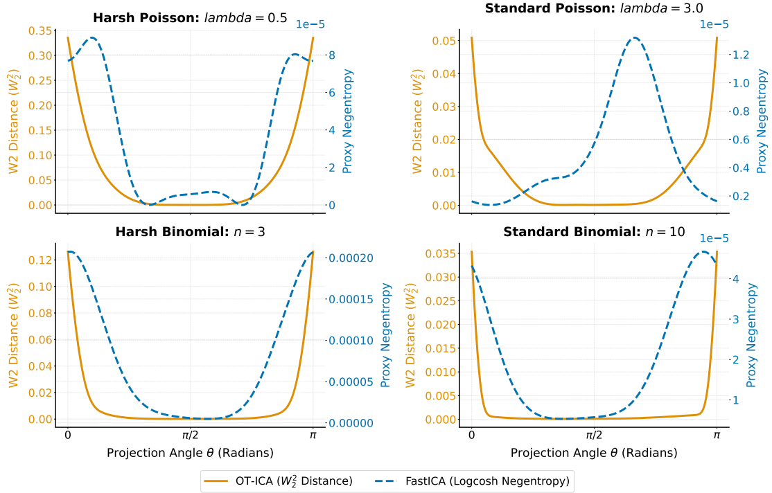
Figure 5.7: The 1D optimization landscapes. The step-function geometry of discrete data creates flat plateaus where the OT-ICA gradient evaluates to zero.
