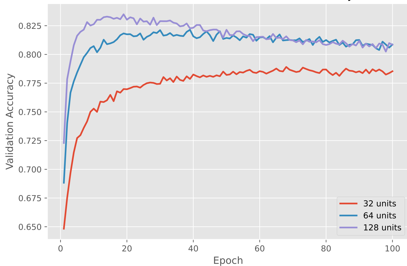
Effect of Network Width on Validation Accuracy
