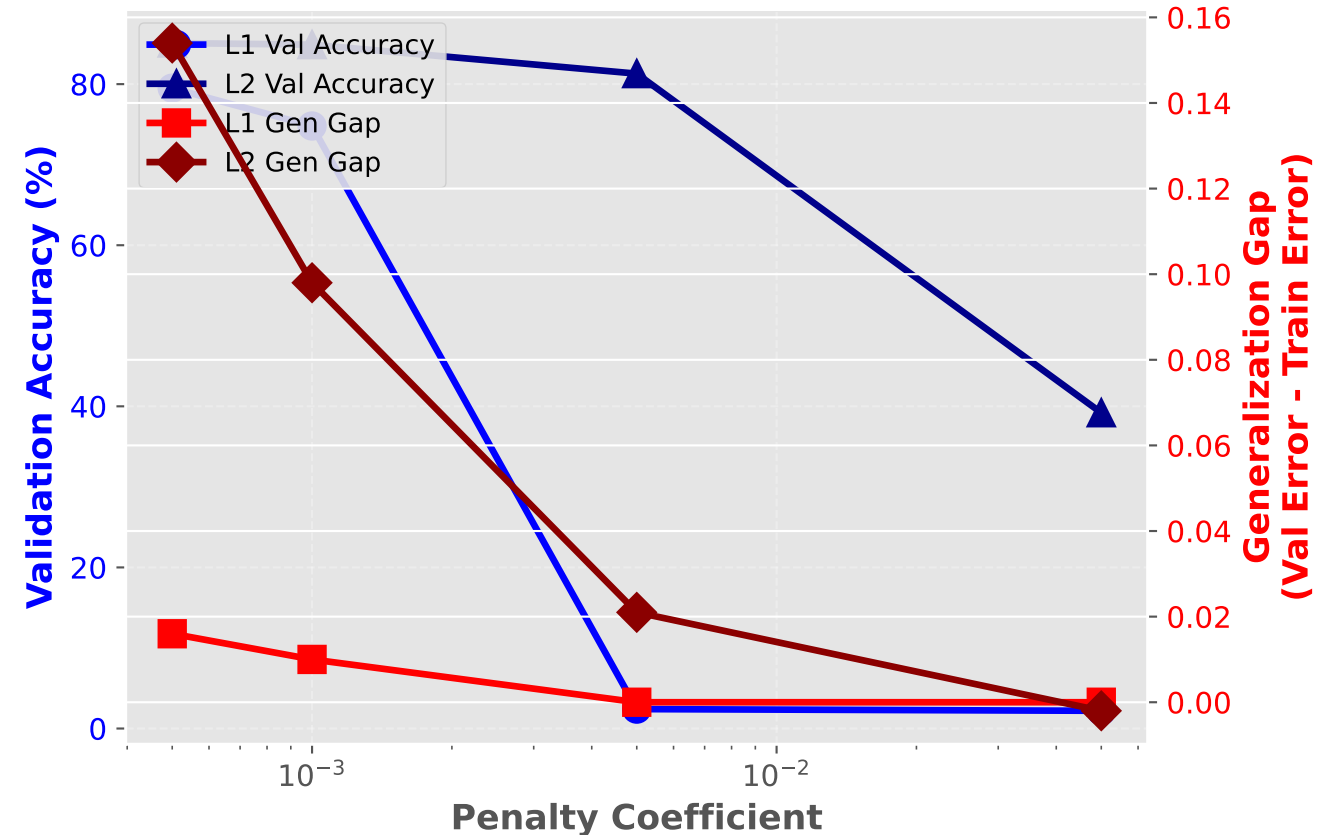
Accuracy and Error by Weight Penalty
