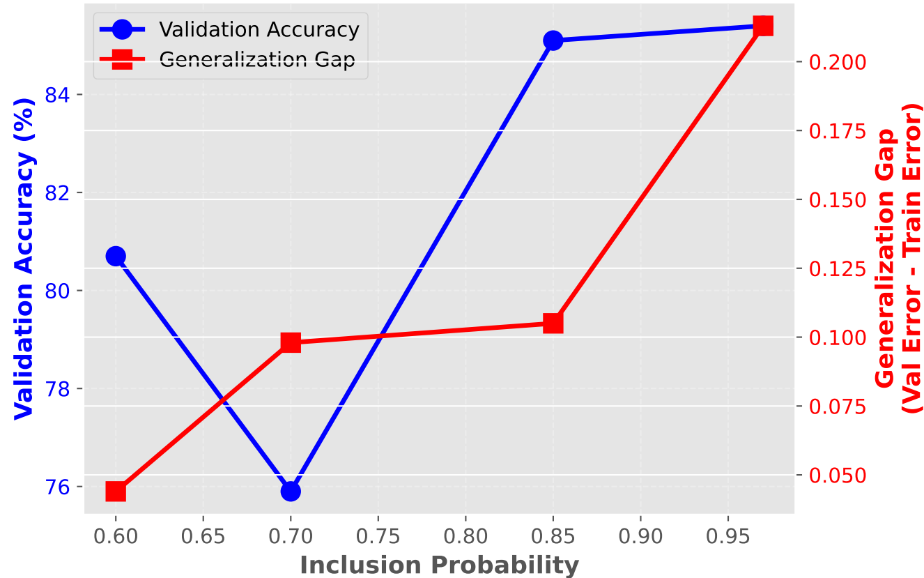
Accuracy and Error by Inclusion Probability
