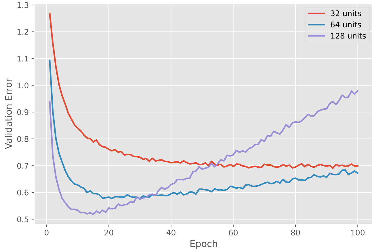
Effect of Network Width on Validation Error
