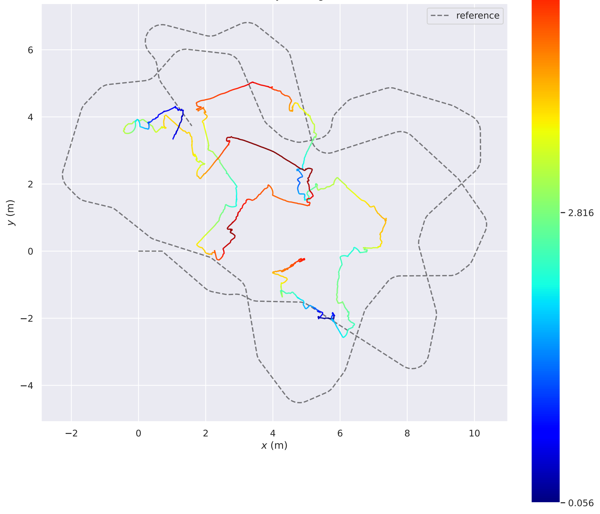
APE w.r.t. translation part (m) (with Sim(3) Umeyama alignment)
