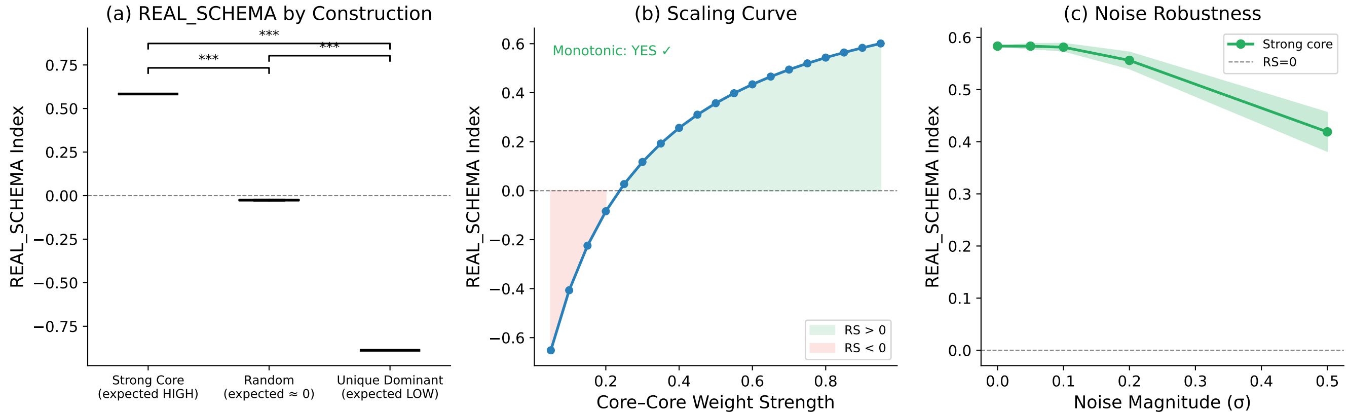
Figure 11: REAL_SCHEMA Synthetic Validation N=100 synthetic networks per case
