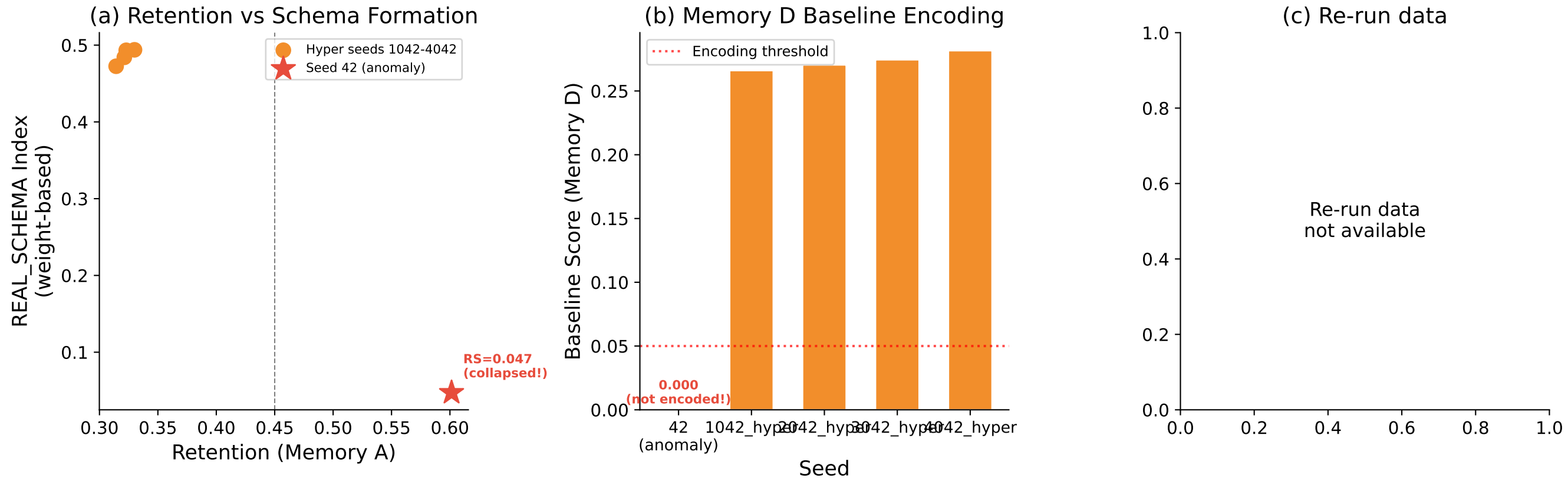
Figure 12: Seed 42 Hyper Replay Anomaly Analysis High retention + collapsed schema = runaway potentiation failure mode
