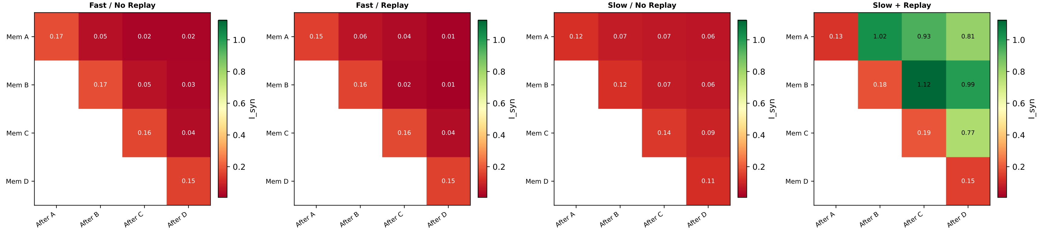
Interference Matrix (rows=probed memory, cols=training checkpoint)
