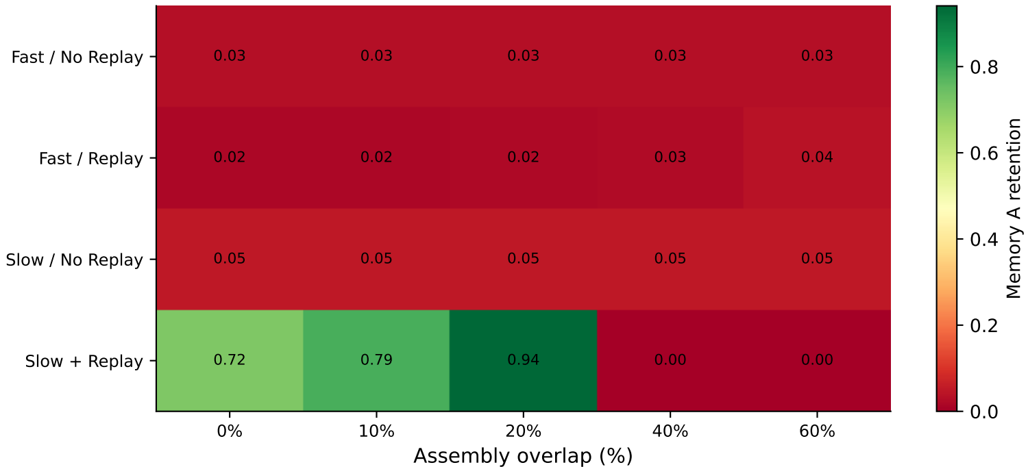
Forgetting Phase Diagram: Overlap x Condition
