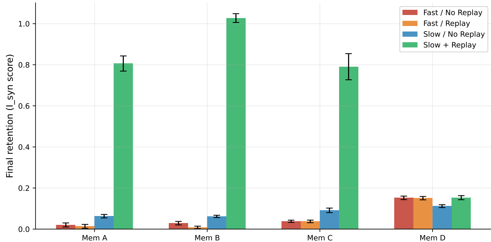
Replay Protection: Final Retention After A->B->C->D
