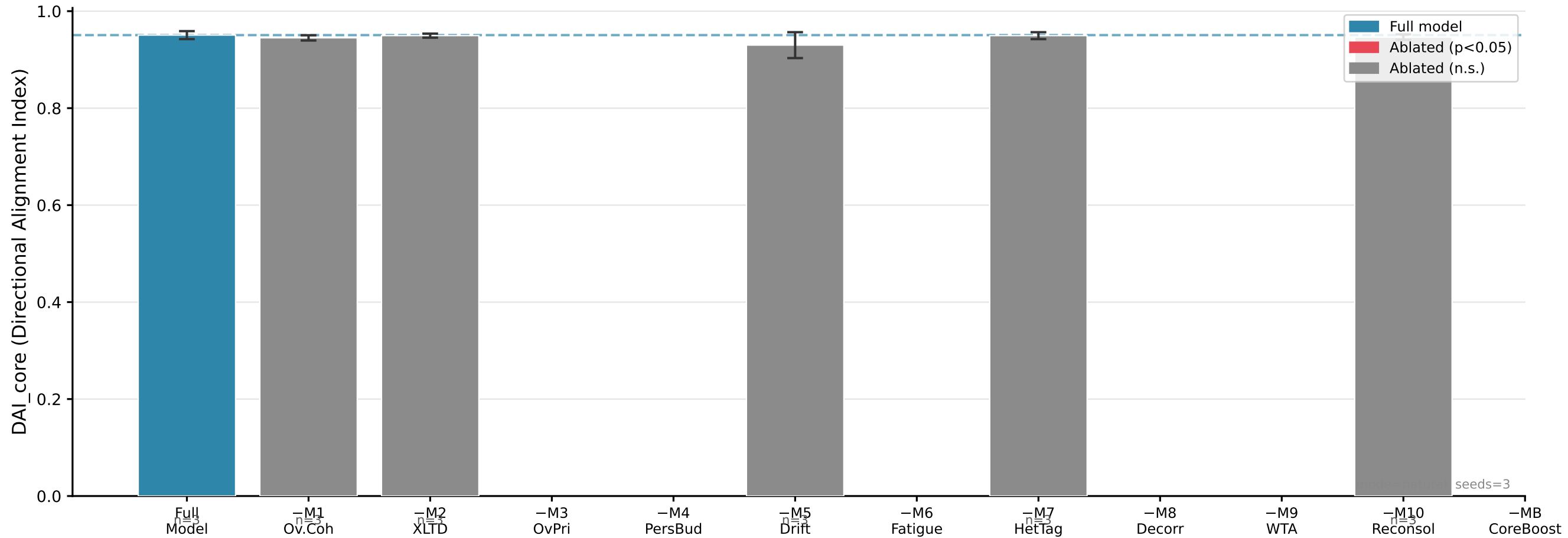
Figure 1: Single-Mechanism Ablations — DAI_core Effect of removing each mechanism on directional schema abstraction
