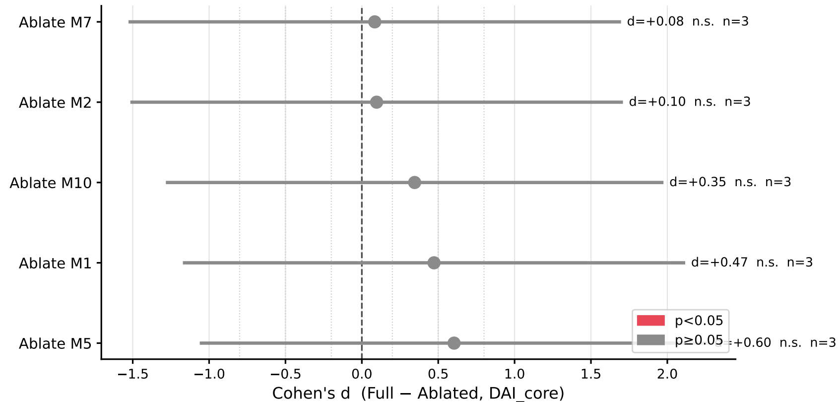
Figure 9: Effect-Size Forest Plot Cohen's d for each single-mechanism ablation (DAI_core)
