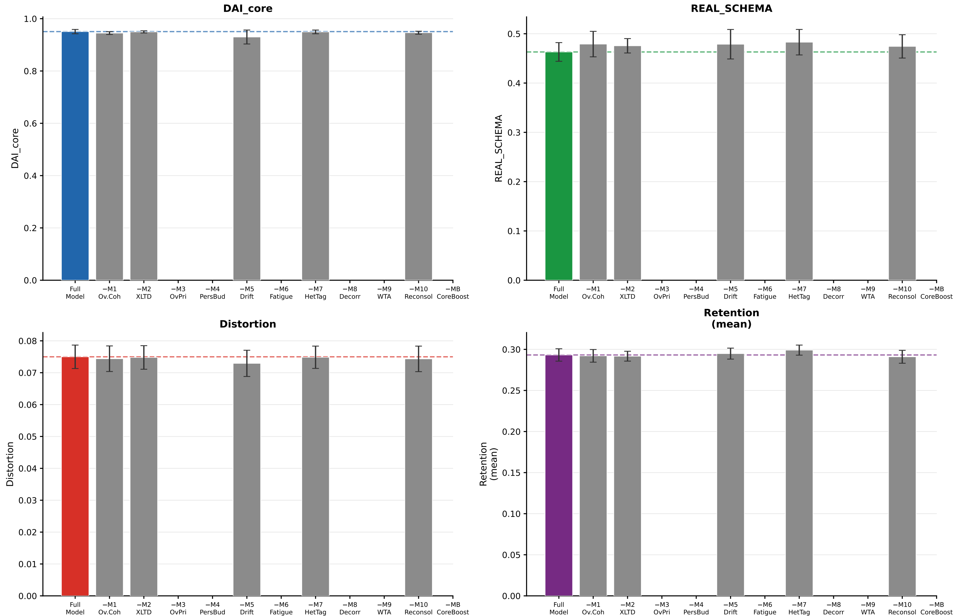
Figure 10: Ablation Study Summary All metrics — single-mechanism ablations
