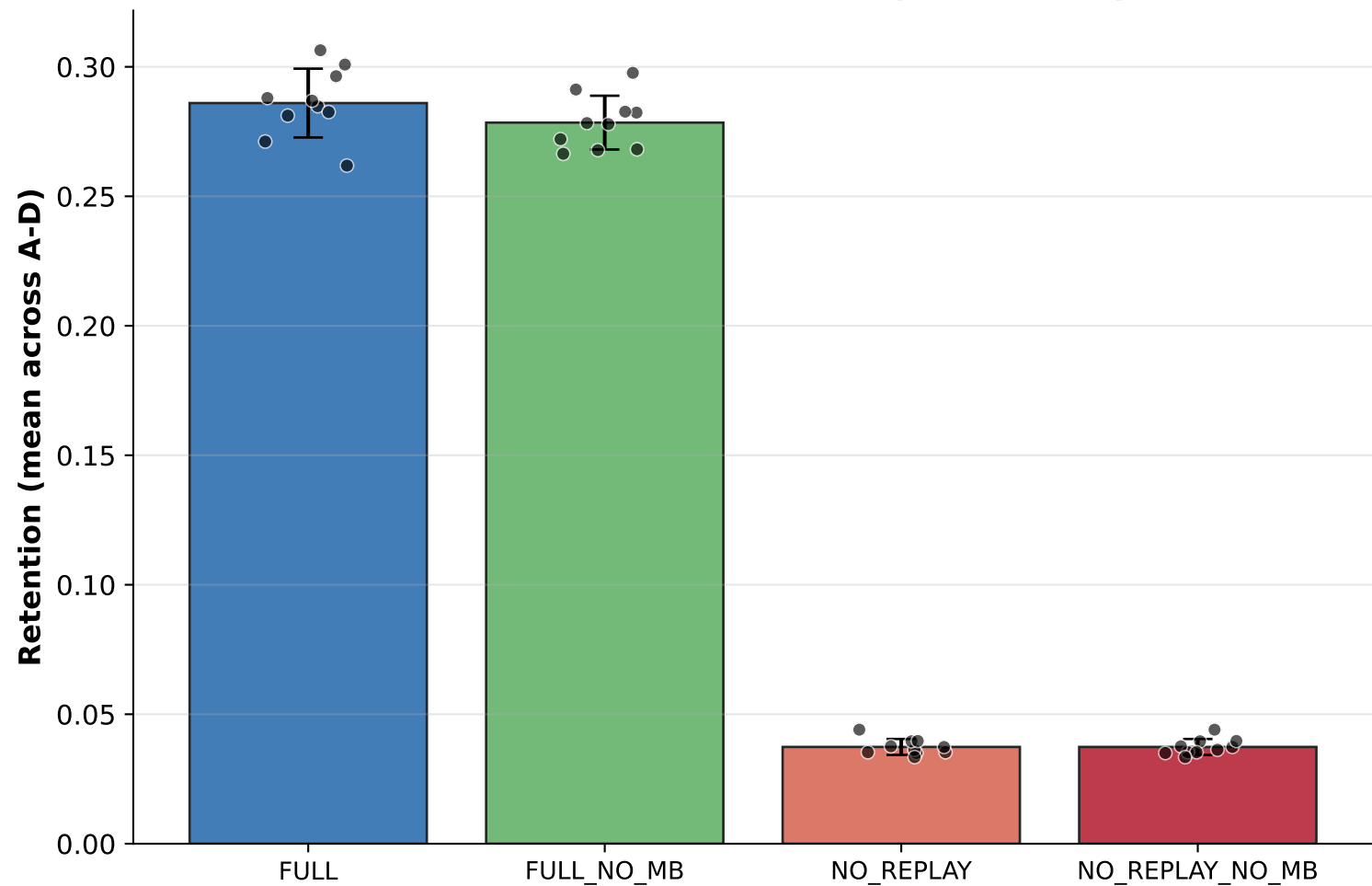
Retention across conditions (n=10 seeds)
