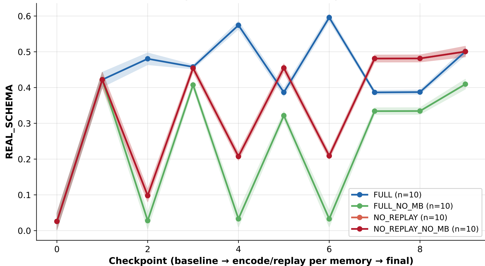
RS evolution over training (mean \pm SEM across seeds)
