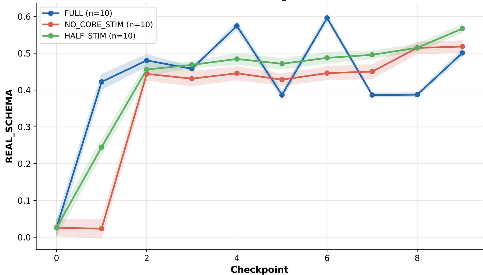
RS evolution over training (mean \pm SEM)
