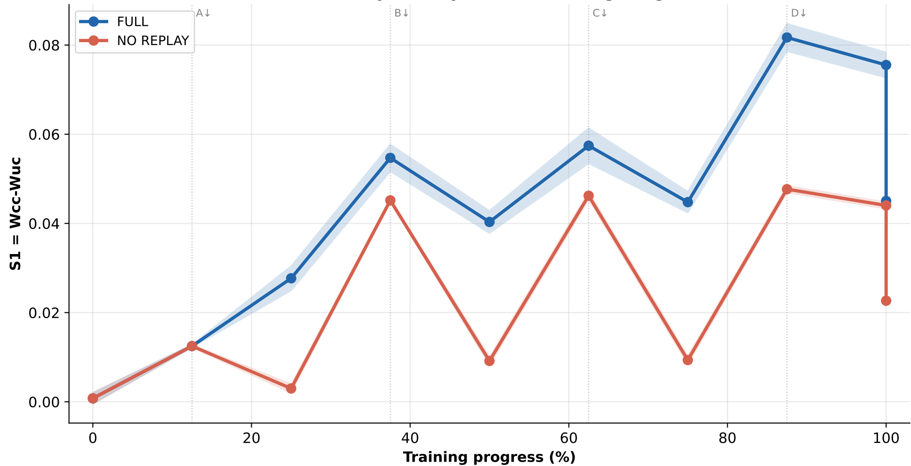
Schema Asymmetry (S1) vs Training Progress
