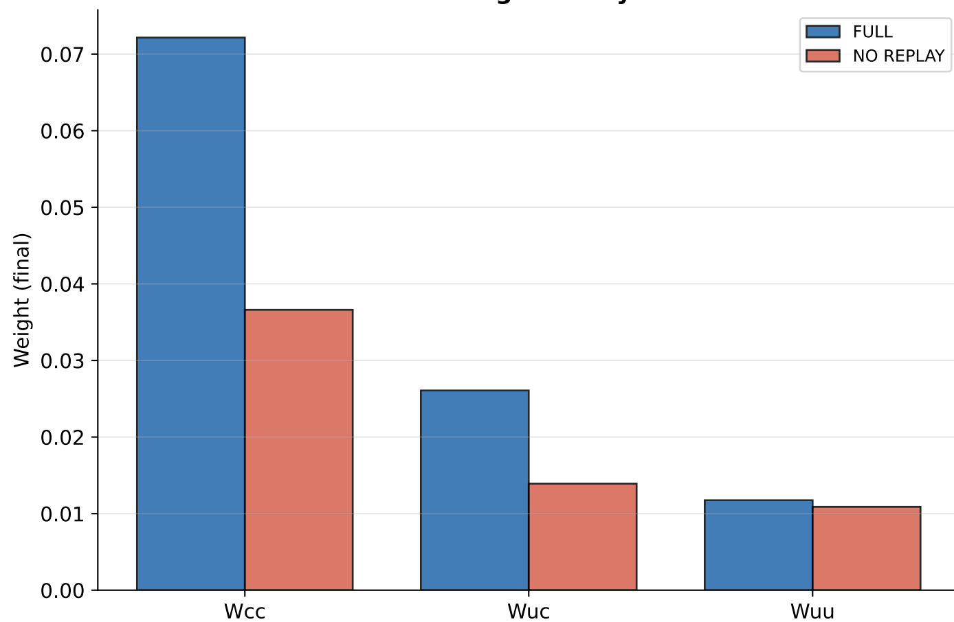
C. Mediation: coincidence -> Wcc ( r=+0.850 , p=0.032 )
