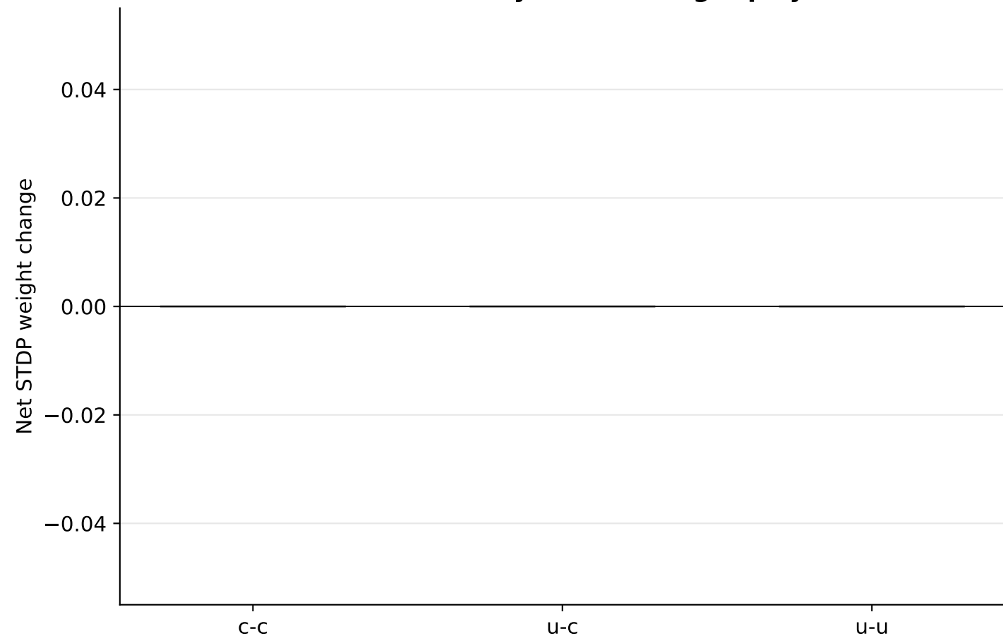
D. Net STDP by block during replay
