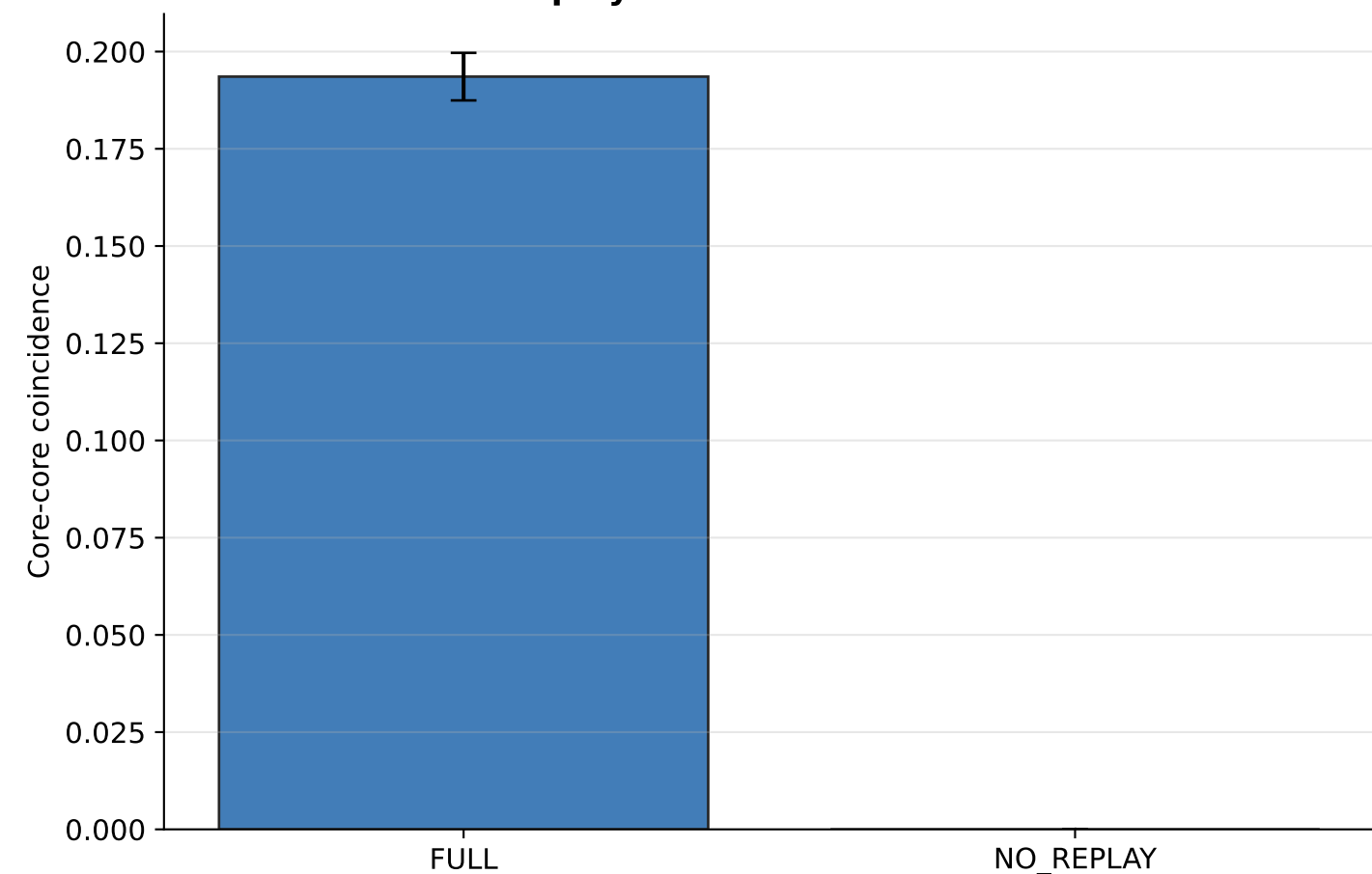
B. Replay drives core coincidence
