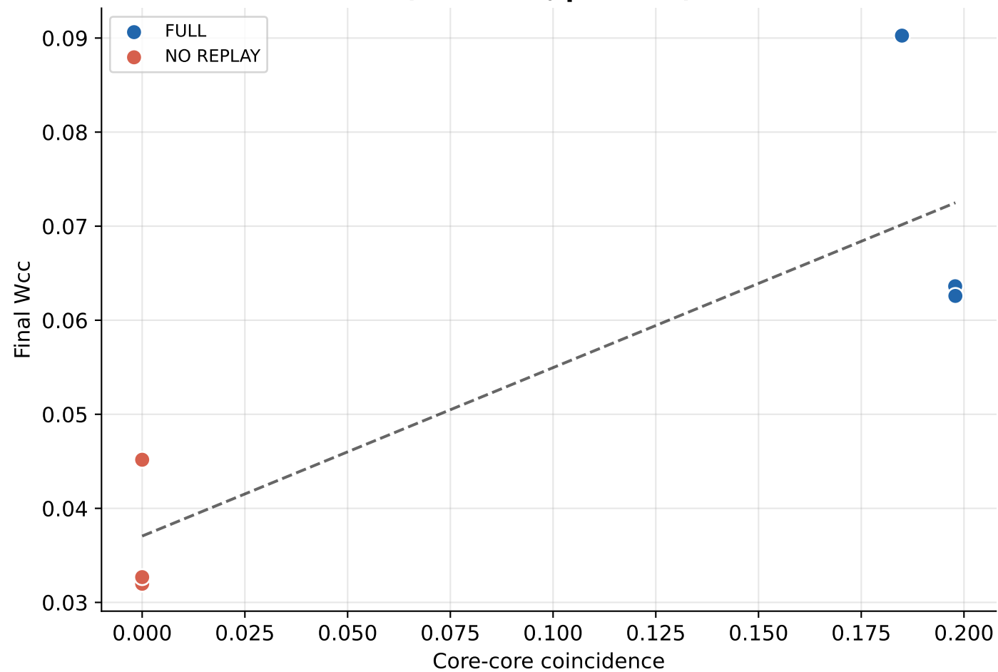
C. Mediation: coincidence -> Wcc ( r=+0.850 , p=0.032 )
